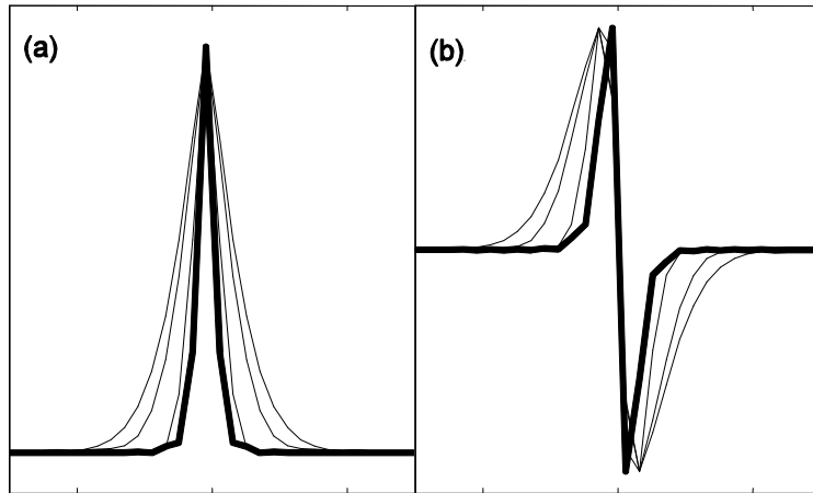
Figure 4: (a) Plot of some optimal post-whitening detectors k(x) , for various values of edge amplitude A , given C=1 and n_o=0.8 . The thick lined profile is the matched detector. The wider detectors are for intermediate values of A . The plots are 30 pixels wide. (b) Plot of corresponding edge detectors f(x) , which are whitened versions of the detectors k(x) . The thick-lined edge detector is the DISEF filter (Equation 22) which corresponds to the matched post-whitening detector in (a).
