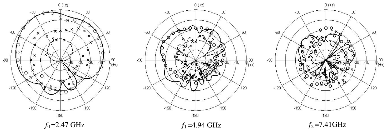
Figure 4: Measured and simulated radiation patterns of the proposed GA-optimised HSA with full-width shorted wall for 2.47 GHz, 4.94 GHz and 7.41 GHz over: z - x plane; (‘—’ measured E_\theta , ‘---’ simulated E_\theta , ‘- - -’ measured E_\phi , ‘xxx’ simulated E_\phi ).
