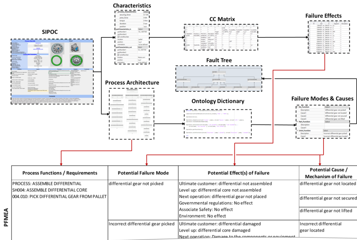
Figure 6. MBSE output information flow into PFMEA
