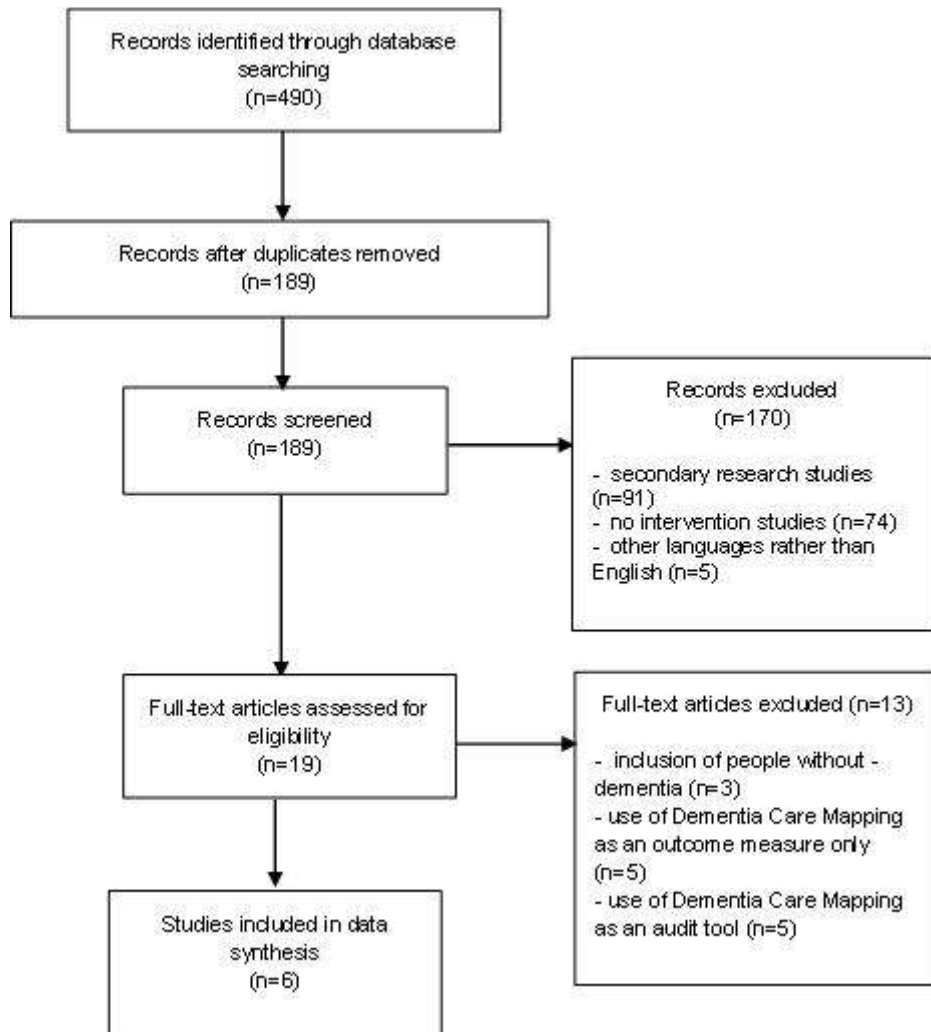
Figure 1. PRISMA diagram
