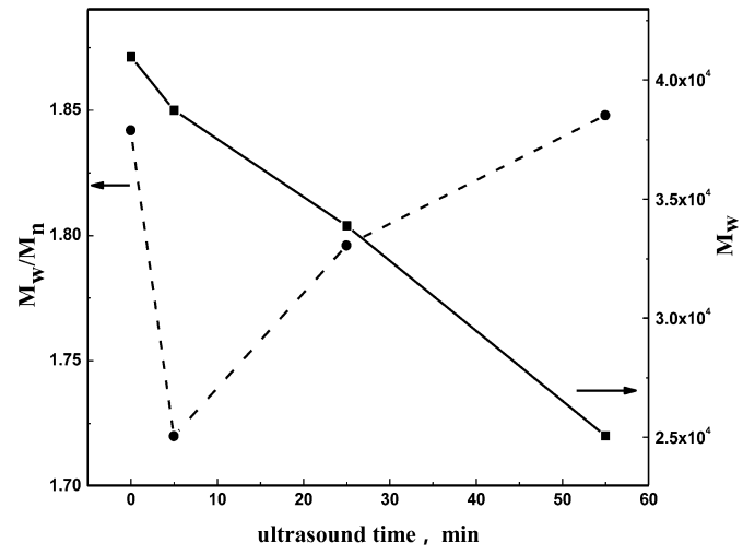
Figure 5 Effect of ultrasound time on M_w and M_w/M_n for PLA (treating temperature: 170°C)
