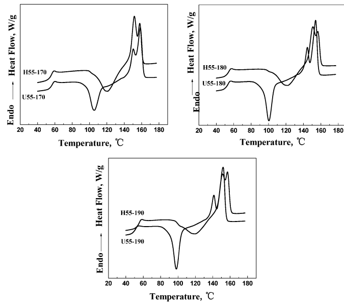
Figure 9 DSC curves of PLA samples prepared by different methods at different temperatures (H55: the PLA samples were treated only by heating for 60minutes; U55: the PLA samples were preheated for 5minutes and then treated by heating and ultrasound for 55minutes)
