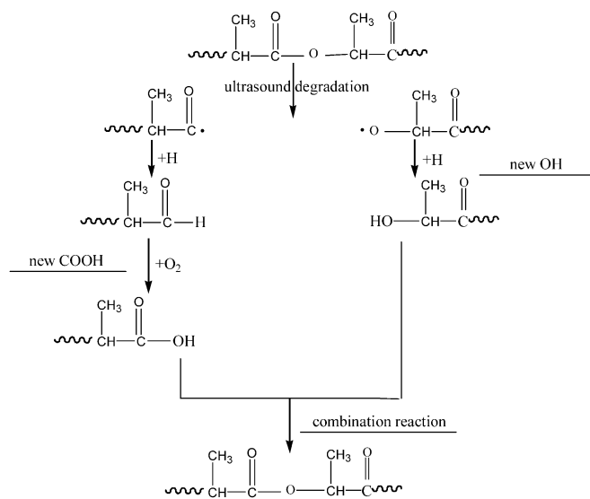
Figure 8 Mechanism scheme for the molecular structure development of PLA under ultrasound
