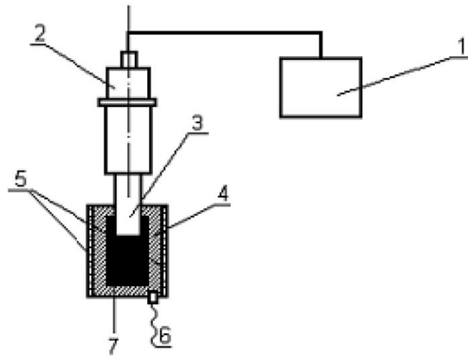
Figure 1 Scheme of the special ultrasound-assisted treater 1: Ultrasound generator; 2: Piezoelectric transducer; 3: Horn; 4: Die; 5: Electric heaters; 6: Thermocouple; 7: Melt
