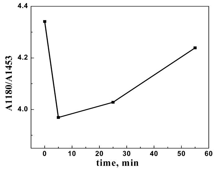
Figure 7 Dependence of A1180/A1453 on ultrasound time (treating temperature: 170°C)
