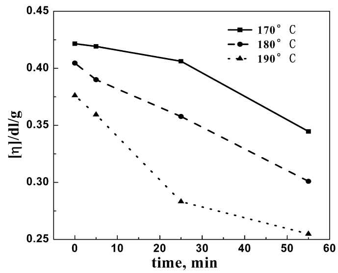
Figure 4 Dependence of [\eta] of PLA on the ultrasound time at different temperatures
