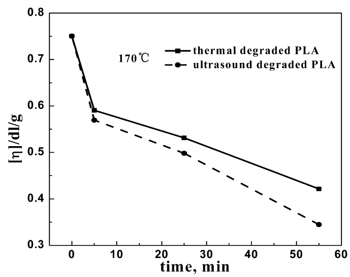
Figure 3 Effect of ultrasound on [\eta] of PLA
