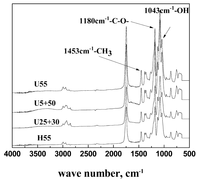
Figure 6 FT-IR spectra of PLA treated at 170°C (U55: treated by ultrasound for 55 minutes; U25+30: treated by ultrasound for 25 minutes; U5+50: treated by ultrasound for 5 minutes; H55: treated only by heating)
