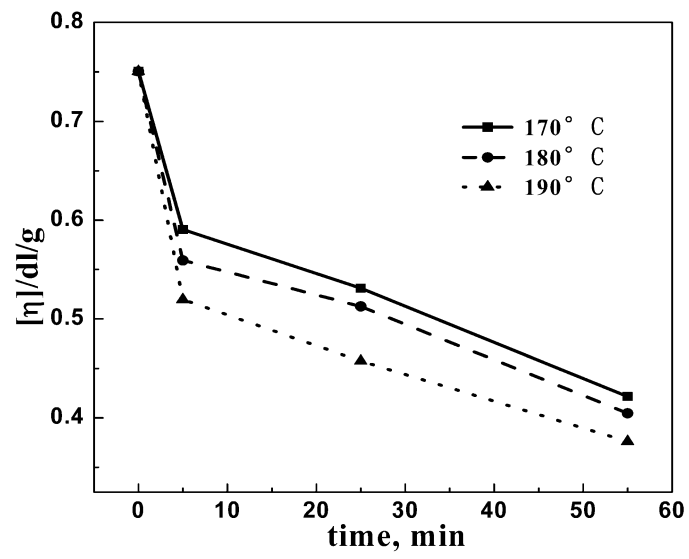
Figure 2 Effect of heating temperature and heating time on [\eta] of PLA
