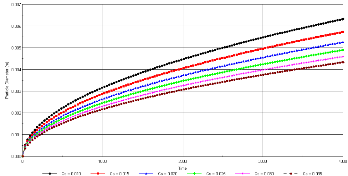
Fig. 17 Variation of crystal particle diameter versus time at different mass fraction of salt in brine feed
