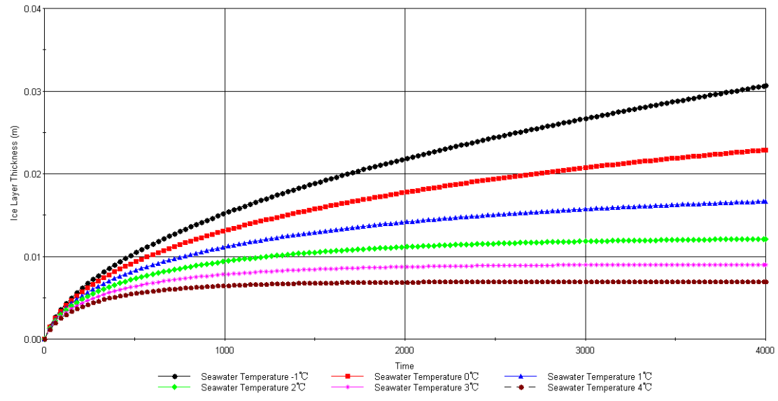
Fig. 16 Variation of the ice layer thickness versus time at different seawater temperatures
