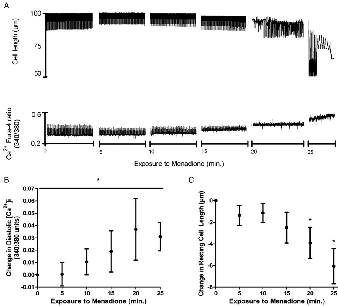
Figure 5. (A) Representative recording of cell length (upper trace) and [Ca 2+ ] i (lower trace) in a single myocyte exposed to 50 μM menadione and stimulated at 1 Hz. Traces represent 1 min recordings at 5 min intervals. (B) Increase in diastolic [Ca 2+ ] i and (C) decrease in resting cell length during exposure to menadione. * P < 0.05, 1-way RM ANOVA vs. pre-exposure; n = 7 myocytes from n = 4 hearts.
