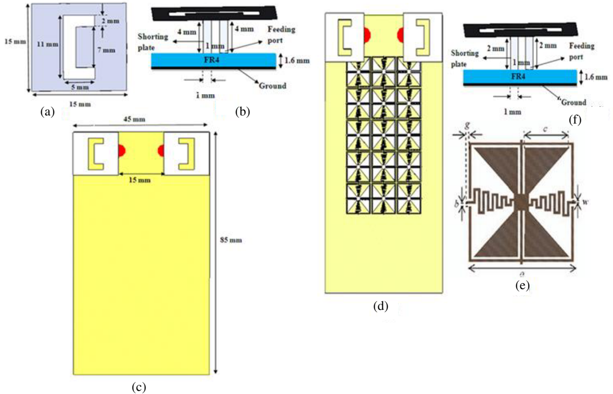
Figure 1: Geometries and dimensions: U-shape antenna (a) top view, (b) side view, (c) 2-D schematic; U-shape antenna with EBG (d) 2-D schematic, (e) EBG unit cell, (f) side view.
