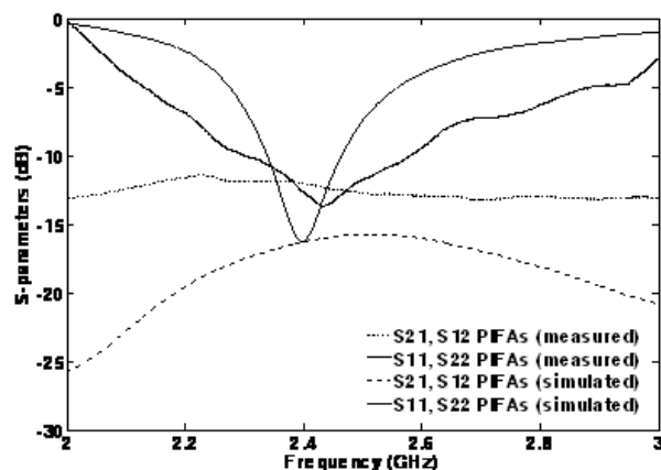
Figure 2: Comparative plot of s -parameters output for simulated and measured results for PIFAs without EBG.
