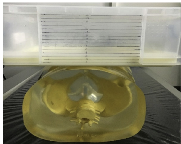
Figure 1. Experimental setup of the pelvis phantom and additional fat container (scaled 1 cm increments in a plastic box).
