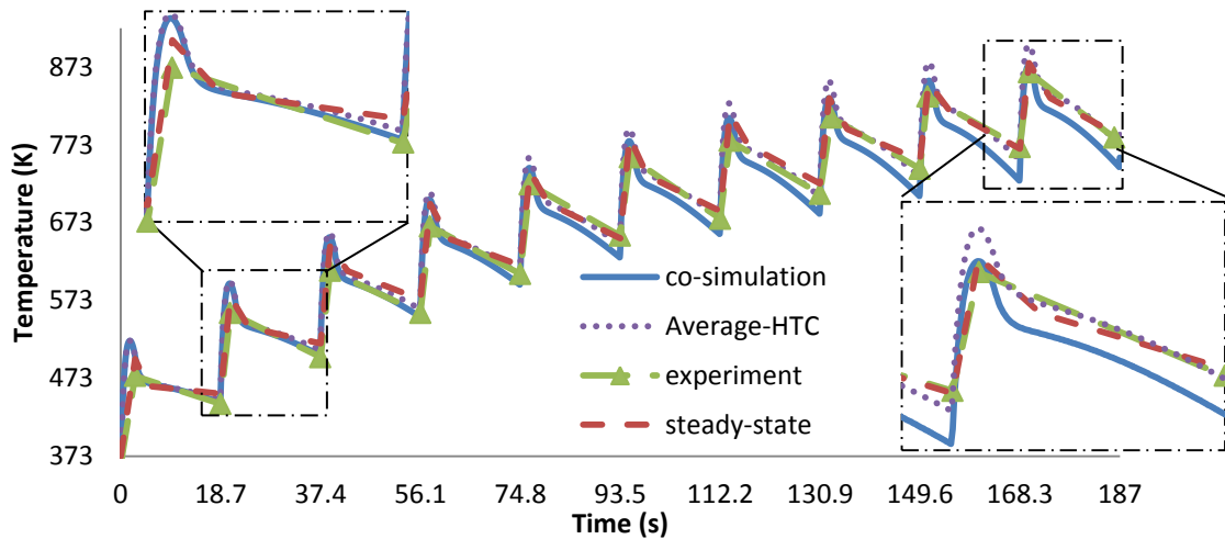
Figure 14: Co-simulation, steady-state method and experiment disc maximum temperature evolution time course
