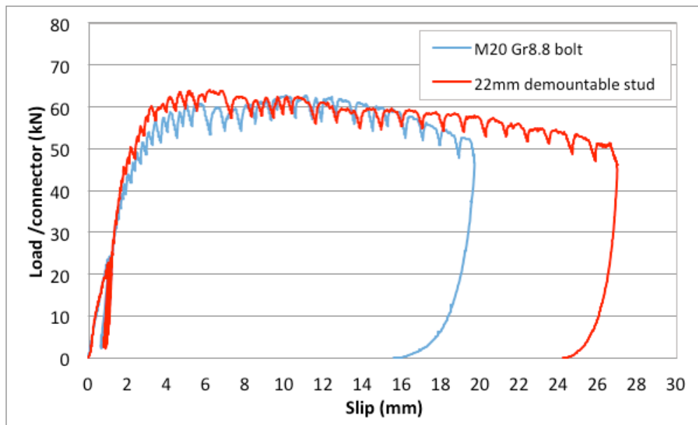
Figure 6: M20 bolt vs. 22mm demountable stud
