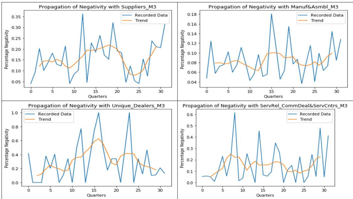
Figure 4: Negativity propagation
