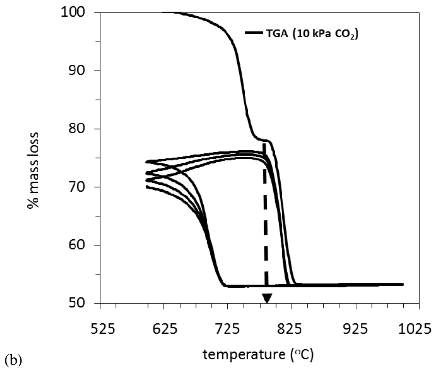
Figure 4. (a) CO 2 concentration (scatter points) and reactor temperature (line) with time. First peak corresponds to the MgCO 3 decomposition; second peak is the CaCO 3 decomposition in macro- scale ('dry') (b) micro- scale (same conditions) temperatures (the arrow indicates the initial temperature of the first thermal decomposition of CaCO 3 ).
