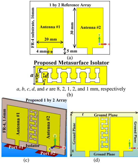
Fig. 1. Configuration of (a) reference array antennas, (b) proposed integrated closed isolator based on metasurface, (c) proposed array antennas applying the proposed decoupling slab, and (d) ground-plane of both structures, f and g are 60 mm & 40 mm, respectively.
