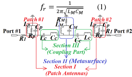
Fig. 3. Equivalent circuit diagram of the proposed 1x2 array antenna.
