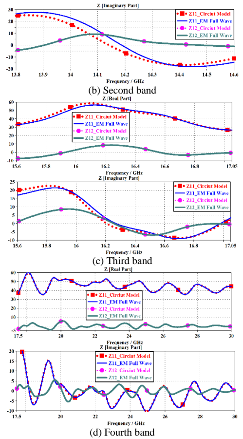
Fig. 4. Input impedances ( \Omega ) & admittances ( 1/\Omega ) of the proposed array.
