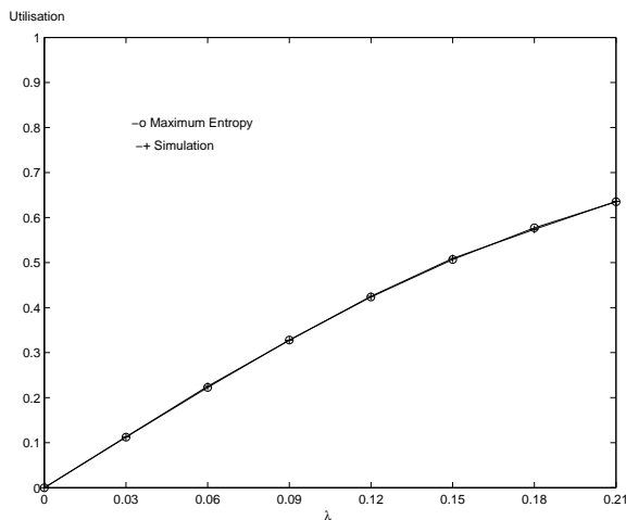
Figure 5: Utilisation of the layer 3
