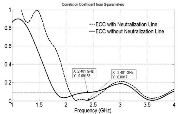
Figure 9. Simulated envelope correlation coefficient for the proposed antenna with and without neutralization line.
