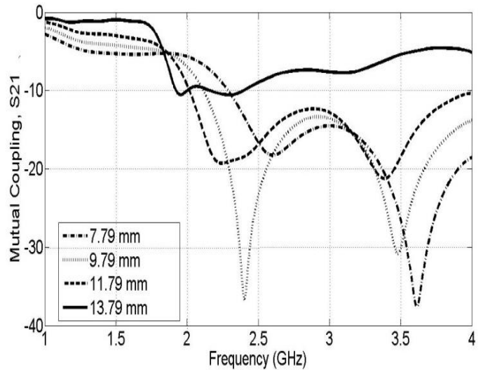
Figure 2. Simulated transmission coefficient, S_{21} of the various distance location of neutralization line.
