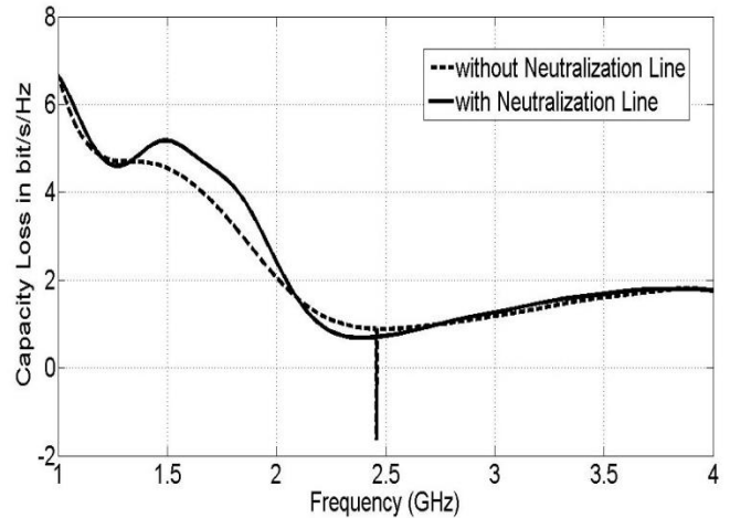
Figure 11. Simulated capacity loss of the proposed antenna with and without neutralization line.
