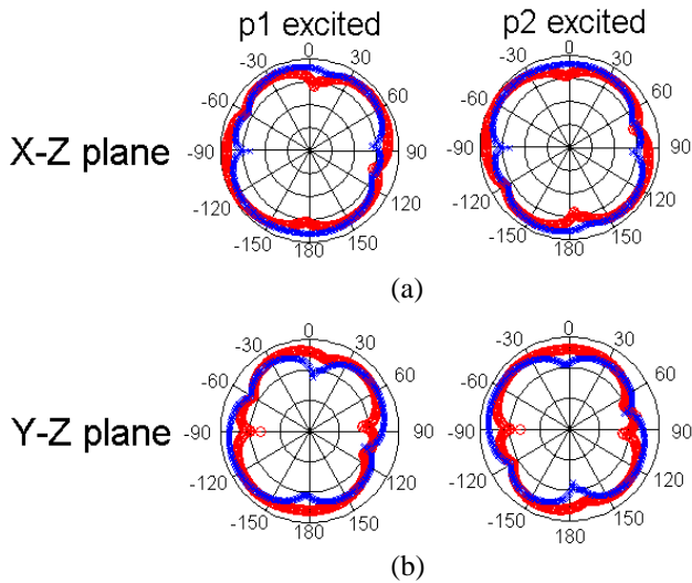
Figure 7. Simulated radiation patterns for the proposed antenna for two planes at 2.4 GHz; (a) X-Z plane. “xxxx” (blue) simulated cross-polarization, “oooo” (red) simulated co-polarization. (b) Y-Z plane. “xxxx” (blue) simulated co-polarization, “oooo” (red) simulated cross-polarization Port 1(left) excited and port 2(right) terminated in 50Ω.
