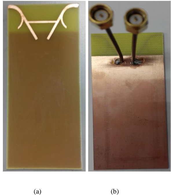
Figure 5. Practical prototype of the proposed antenna (a) top view (b) back view.
