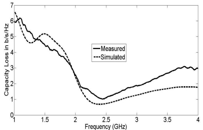
Figure 12. Comparison Between simulated and measured capacity loss of the proposed antenna.
