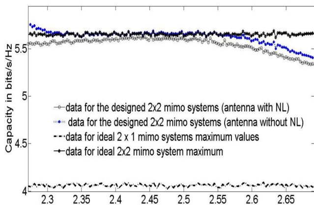
Figure 15. Simulated capacity of the proposed antenna with and without neutralization line.
