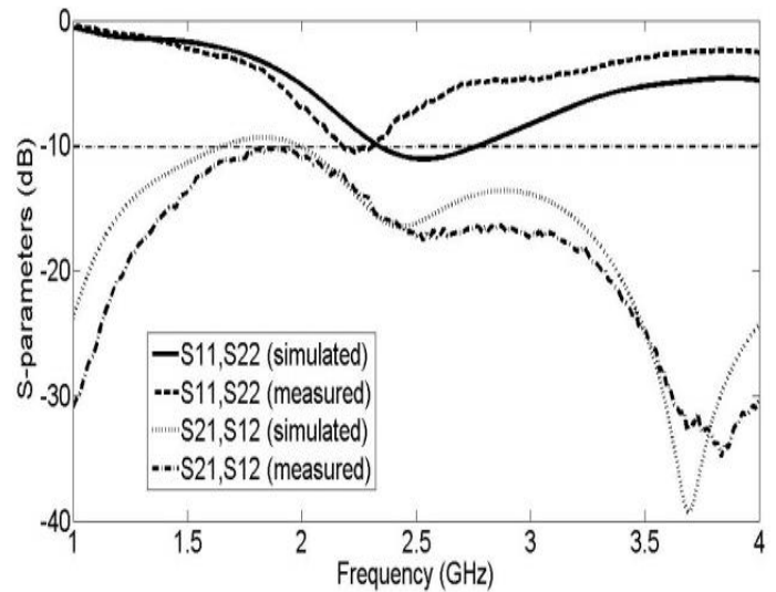
Figure 3. Comparative plot of s-parameters output for simulated and measured results for the proposed antenna without neutralization line.
