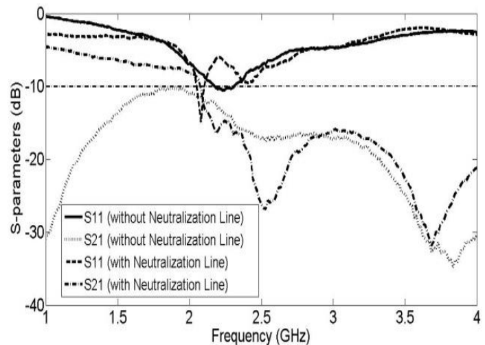
Figure 6. Measured S-parameters of the proposed antenna with and without the neutralization line.
