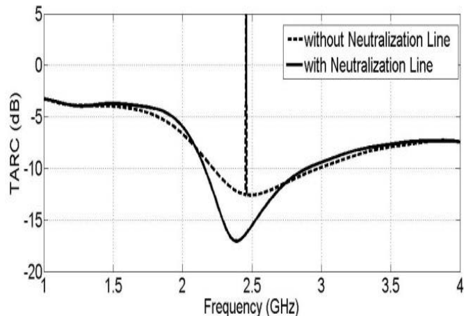
Figure 13. Simulated total active reflection coefficient of the proposed antenna with and without neutralization line.
