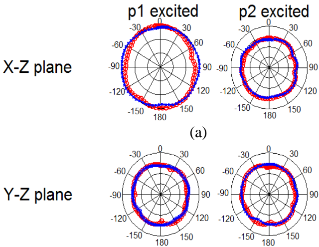
Figure 8. Measured radiatio (b) is for the proposed antenna for two planes at 2.4 GHz; (a) X-Z plane. “xxxx” (blue) simulated co-polarization, “oooo” (red) simulated cross-polarization. (b) Y-Z plane. “xxxx” (blue) simulated cross-polarization, “oooo” (red) simulated co-polarization Port 1(left) excited and port 2(right) terminated in 50Ω.
