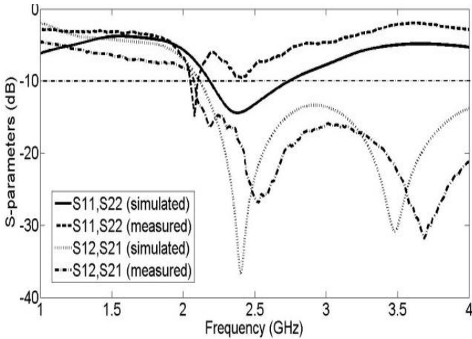
Figure 4. Comparative plot of s-parameters output for simulated and measured results for the proposed antenna with neutralization line.
