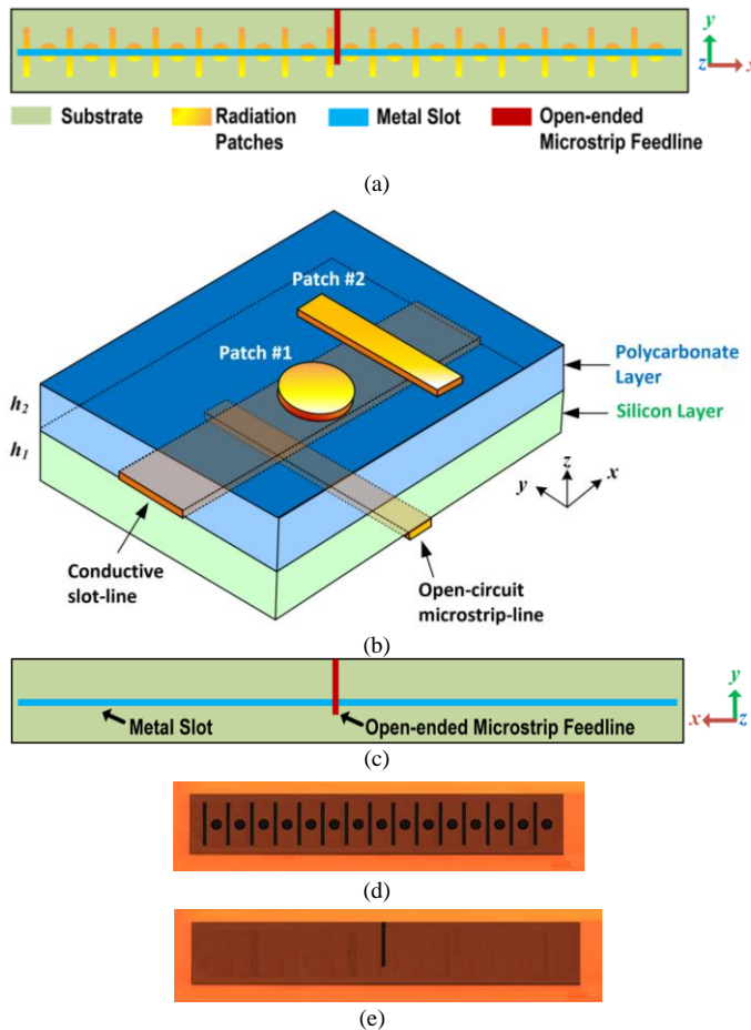
Fig. 1. Silicon-based integrated on-chip antenna, (a) top-side, (b) side-vision with a partially enlarged section, (c) back view, (d) manufactured prototype (top-side), and (e) manufactured prototype (bottom-side). The proposed on-chip antenna has a total dimension of 20 \times 3.5 \times 0.126 \text{ mm}^3 . It is constructed from three different layers, i.e.: (i) polycarbonate, (ii) silicon, and (iii) aluminum.
