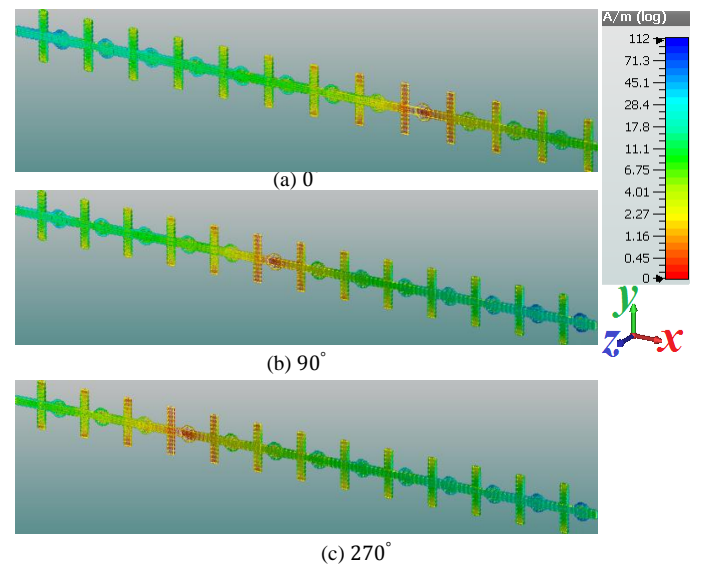
Fig. 3. Surface-current distribution over the radiation elements at 300 GHz for different phase angles.
