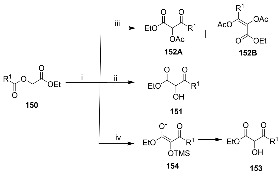
Scheme (58) Reagents and conditions: i) LDA, THF, 0 °C, 30 mins; ii) HCl (0.1 N); iii) Ac 2 O; iv) TMSCl.
