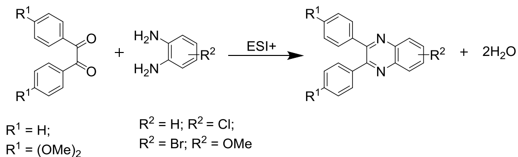
Scheme (42): Formation of quinoxalines under ESI+ condition.
