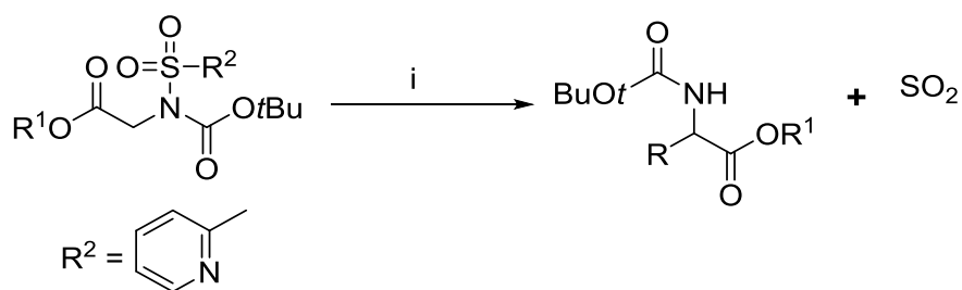
Scheme (63) Reaction and conditions: i) LDA, THF, -78 °C, N 2 .
