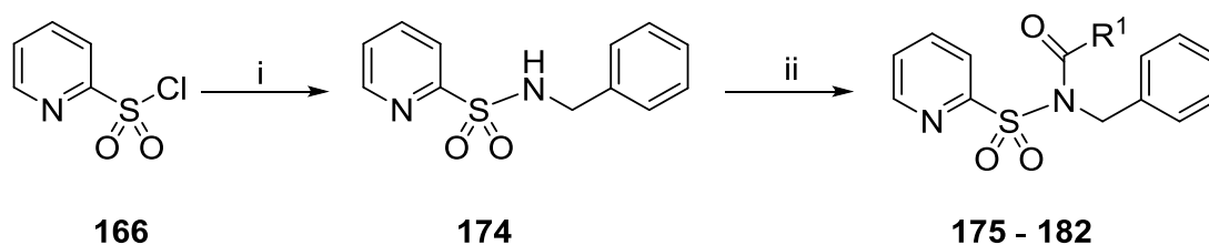
Scheme (67) Reagents and conditions : i) \text{PhCH}_2\text{NH}_2 , \text{Et}_3\text{N} , \text{CH}_2\text{Cl}_2 , 98%; ii) \text{NaH} , \text{THF} , \text{R}^1\text{COCl} , 0 °C to rt or \text{R}^1\text{CO}_2\text{COR}^1 , DMAP, \text{py} .
