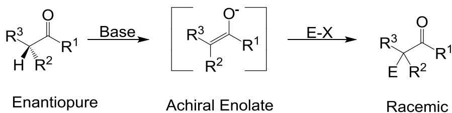
Scheme (60): Reaction of a single enantiomer of a precursor carbonyl compound via the corresponding achiral enolate in the absence of a chiral source.
