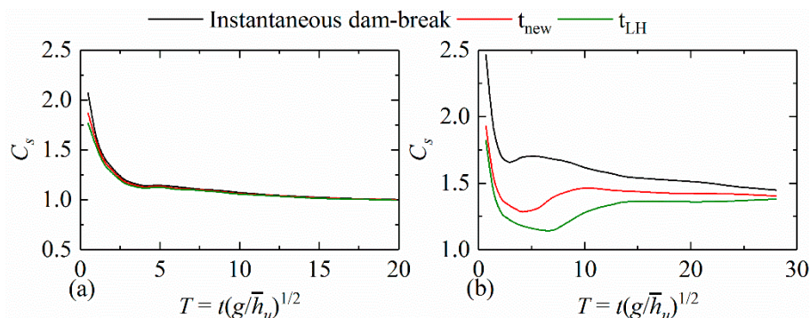
Figure 8. Front velocity for different criterion: (a) A rectangular channel; (b) a triangular channel.
