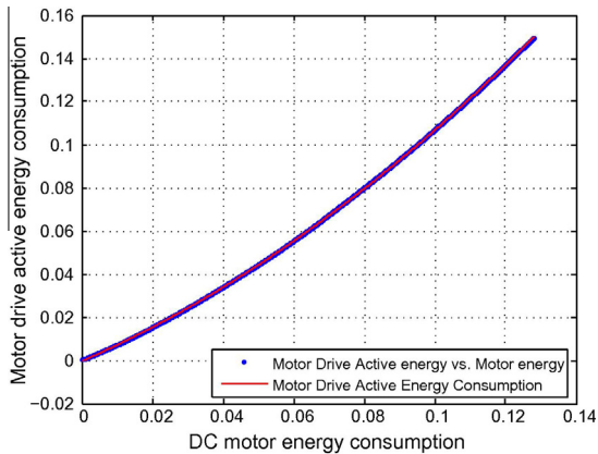
Fig. 7. Approximation of motor drive active energy consumption through 2nd order polynomial model y = 3.6x^2 + 0.71x , the R -square value is 1.
