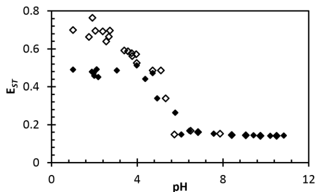
Figure 11. The changing energy transfer of dilute mixtures of P(AA-co-ACE-co-AMMA) (◇) alone and mixed with an equal concentration of PAM (◆) with pH.
