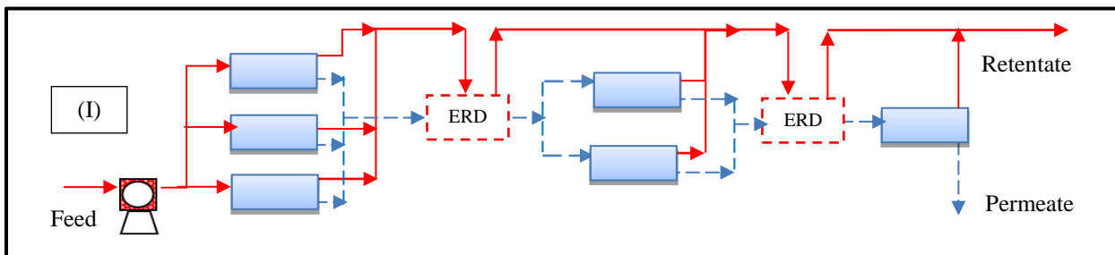
Fig. 2. Tested configuration of permeate reprocessing RO network of three stages
