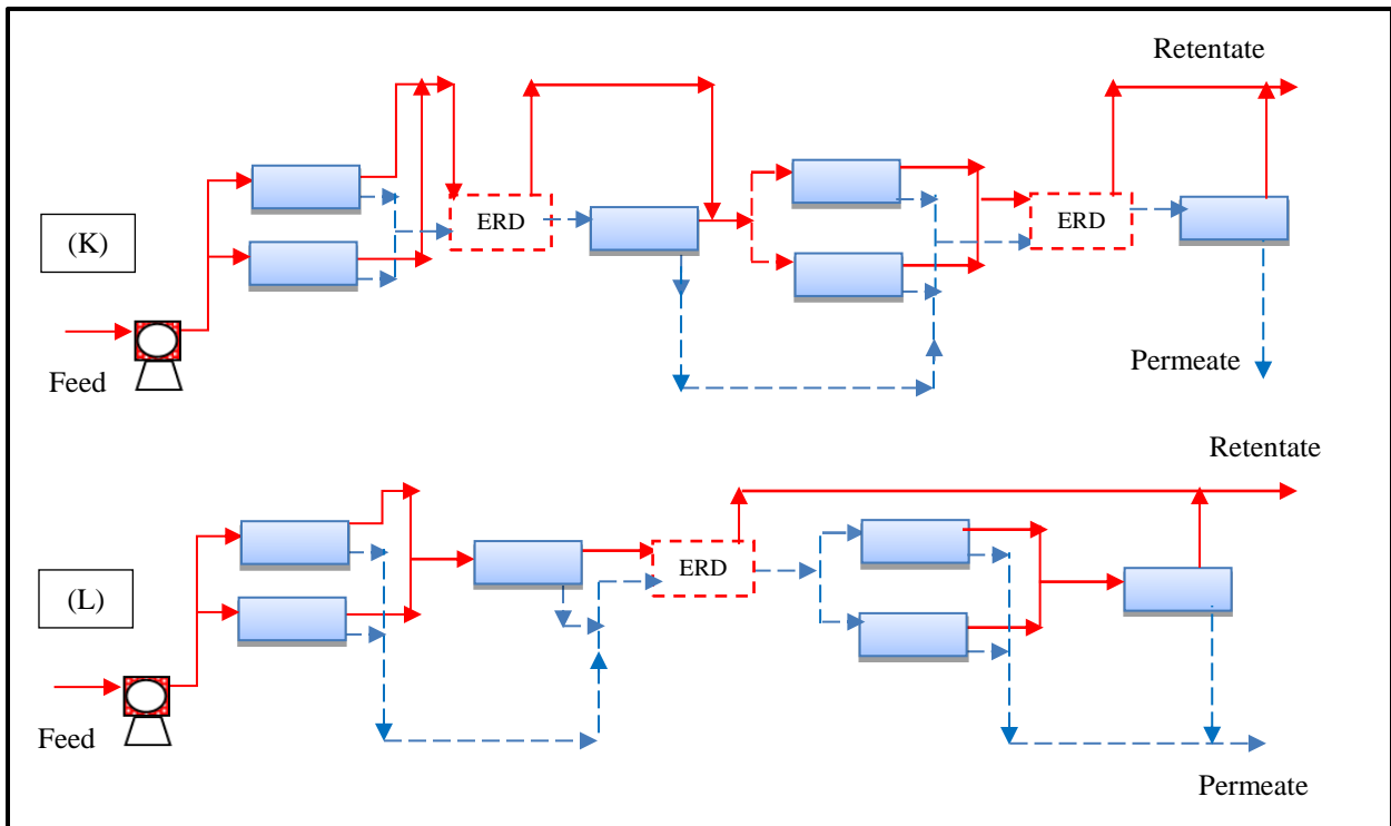
Fig. 4. Tested two configurations of retentate and permeate reprocessing RO network of four stages
