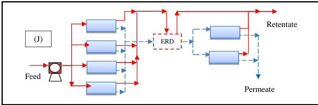
Fig. 3. Tested configuration of permeate reprocessing RO network of two stages
