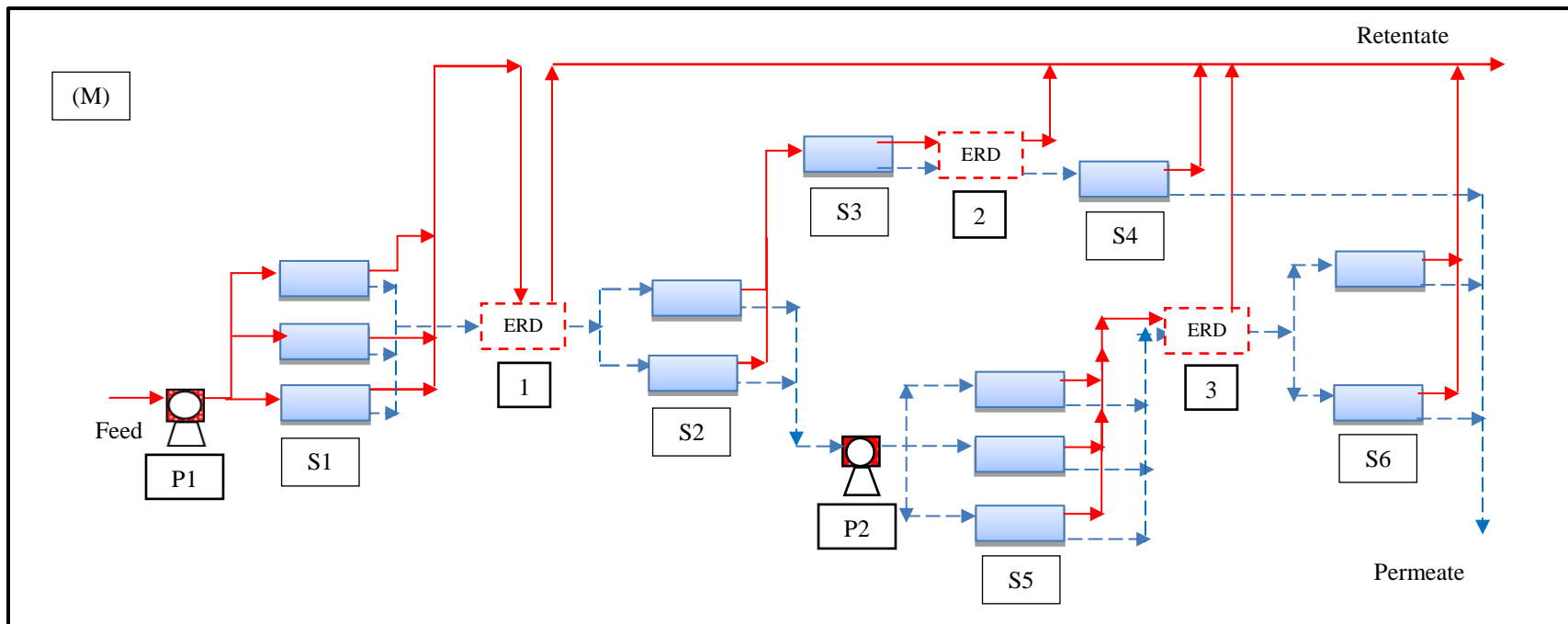
Fig. 5. Six stages RO network with permeate reprocessing, P: Pump, S: Stage, ERD: Energy recovery device
