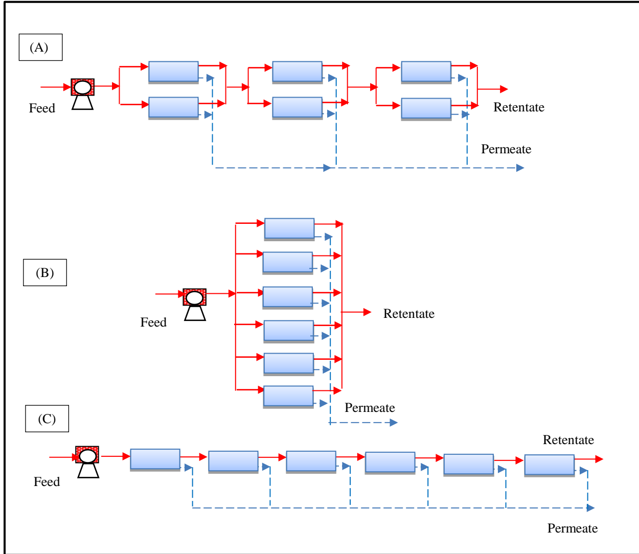
Fig. 1. The tested configurations of retentate reprocessing RO networks of six pressure vessels
