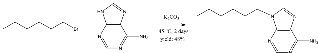
Scheme S1. Synthetic route for the preparation of the adenine-containing mediator.
