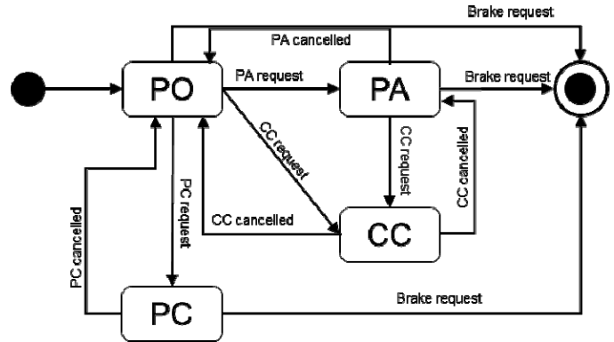
Fig. 4. Statechart of the e-Bike
