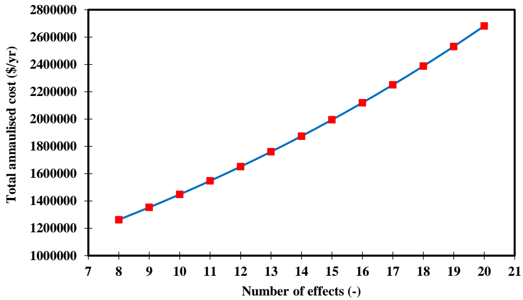
7 Fig. 3. Total annualised cost vs number of effects of MED process at the base case of 39 kg/m 3 of seawater salinity
