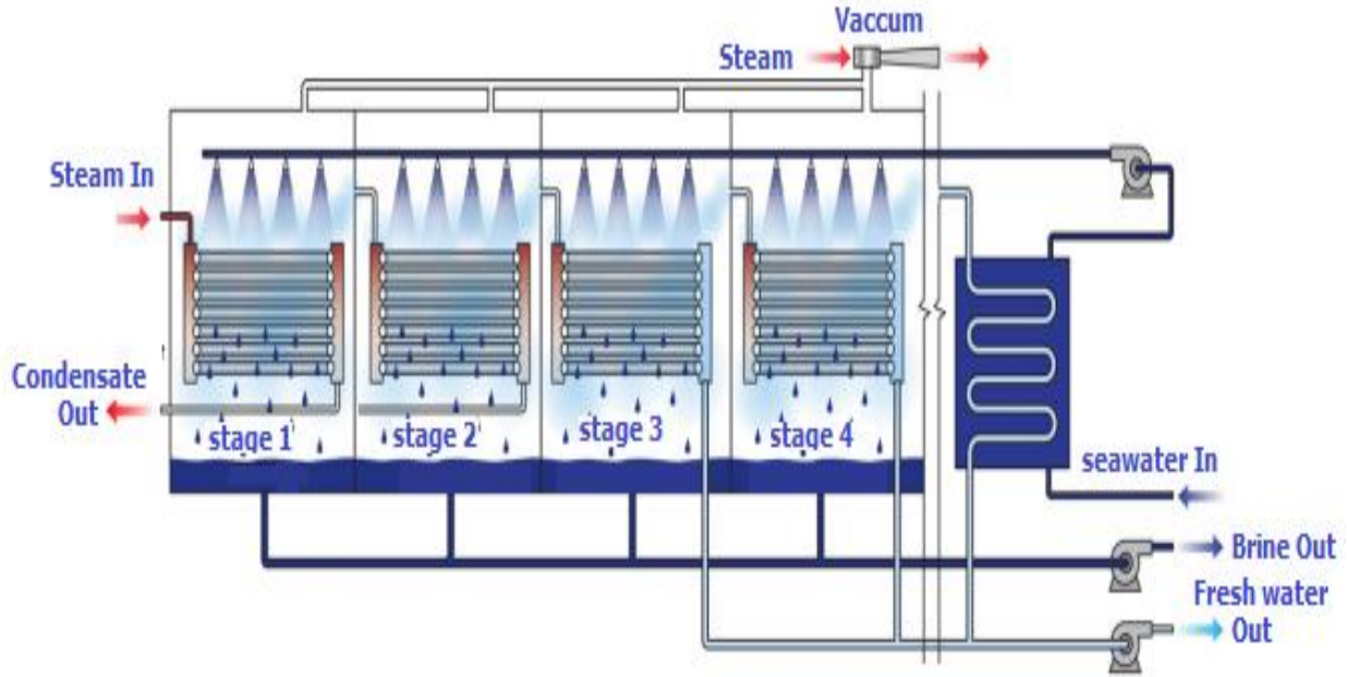
Fig. 1. Schematic diagram of MED system (Adapted from Zak et al., 2012)
