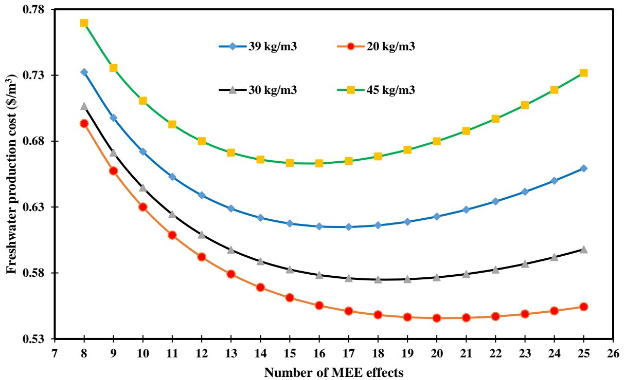
6 Fig. 2. Fresh water production cost vs number of effects of MED process at different seawater salinity
