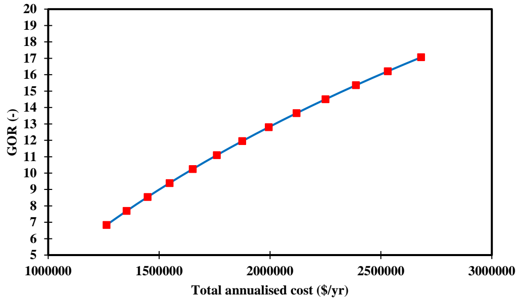
5 Fig 10. Gained Output Ratio vs total annualised cost at the base case of 39 kg/m 3 of seawater salinity
