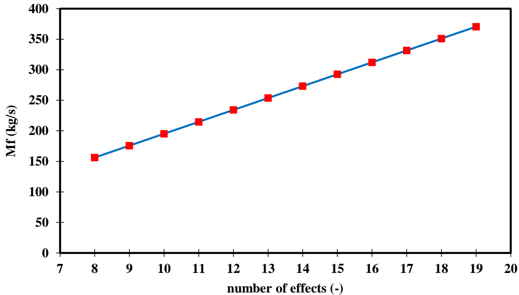
2 Fig. 8. Total seawater feed flow rate vs number of effects of MED process at the base case of 39 kg/m 3 of seawater 3 salinity
