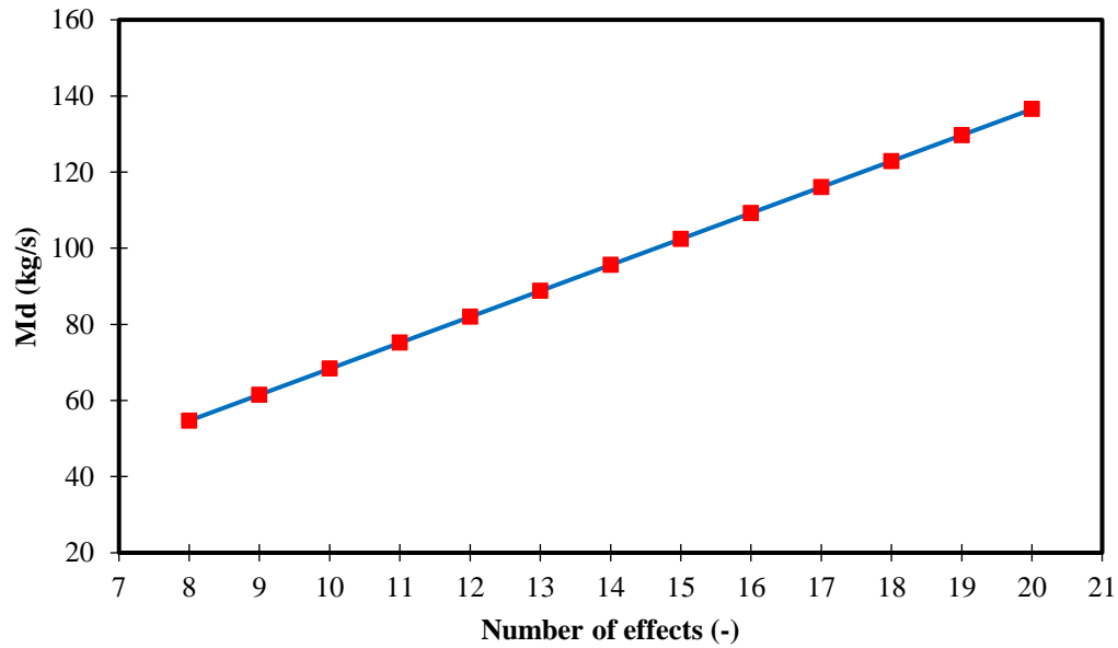
Fig. 7. Total fresh water production flow rate vs number of effects of MED process at the base case of 39 kg/m 3 of seawater salinity
