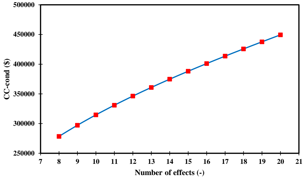
Fig. 6. Final condenser cost vs number of effects of MED process at the base case of 39 kg/m 3 of seawater salinity
