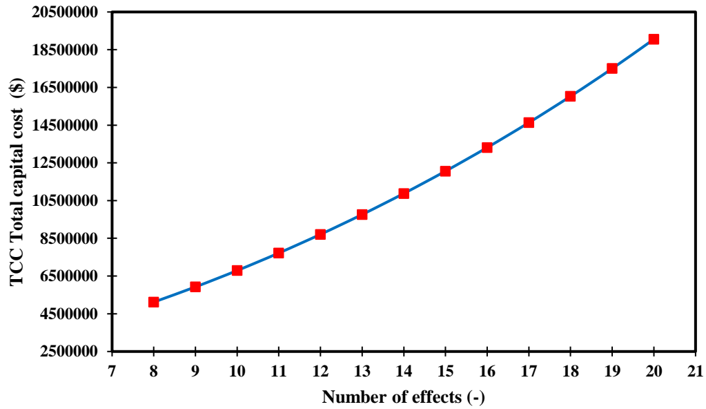
Fig. 4. Total capital cost vs number of effects of MED process at the base case of 39 kg/m 3 of seawater salinity
