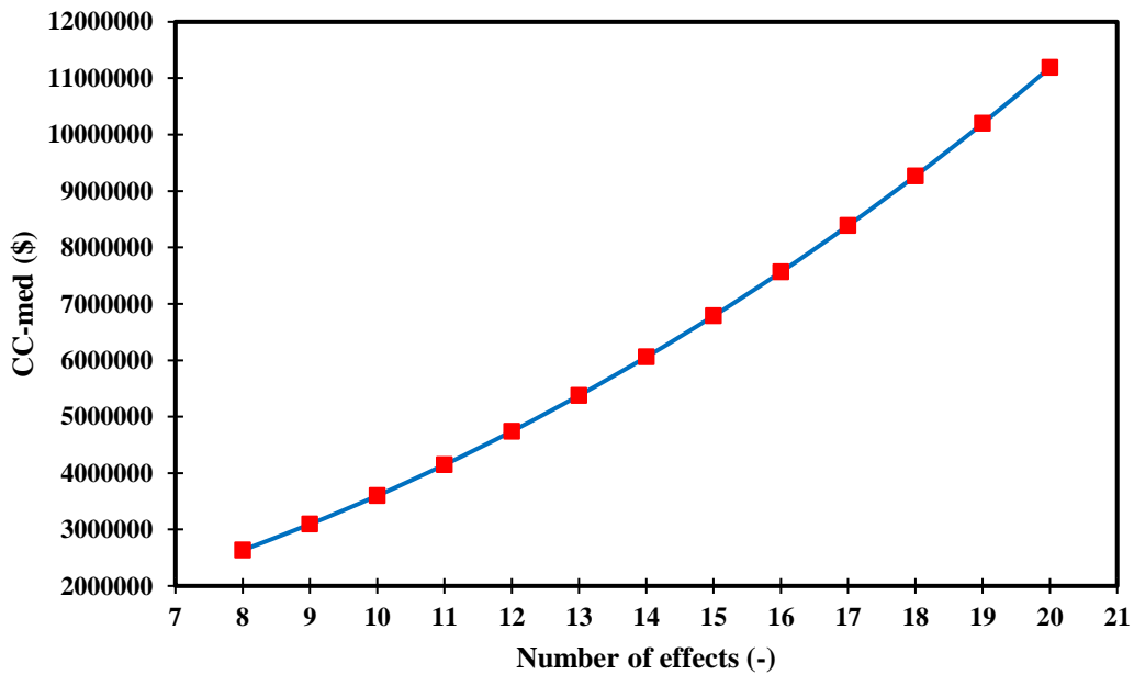
Fig. 5. Total MED plant cost vs number of effects of MED process at the base case of 39 kg/m 3 of seawater salinity
