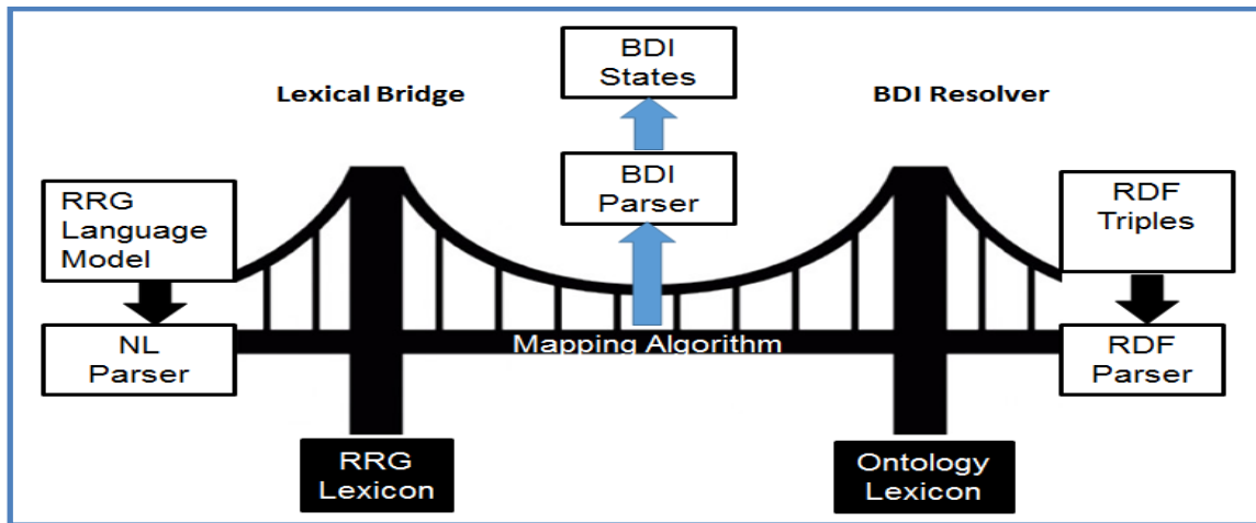
Figure 8: Lexical Bridge for the CSA’s belief base + BDI Parser to resolve the agent’s BDI States (Panesar, 2017)
