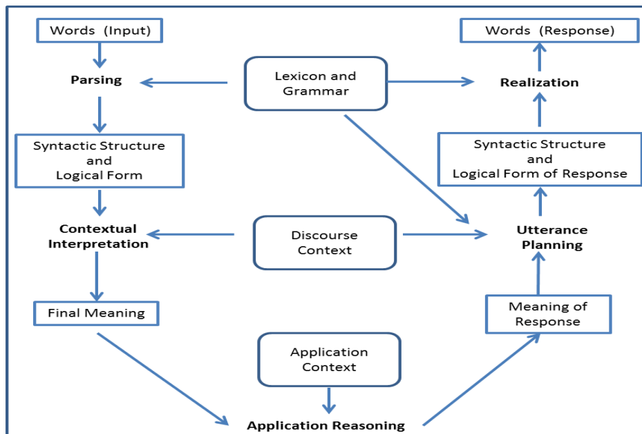
Figure 1: NLP Pipeline.
