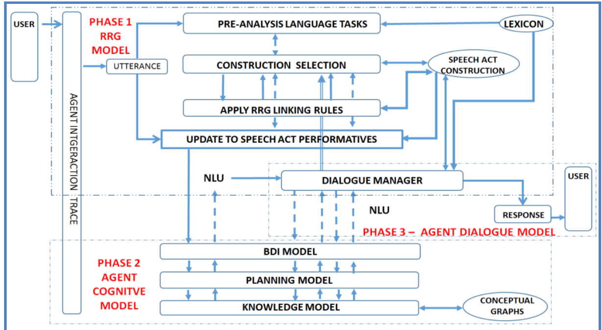
Figure 5: Conceptual Architecture of the Ling-CSA (Panesar, 2017).
