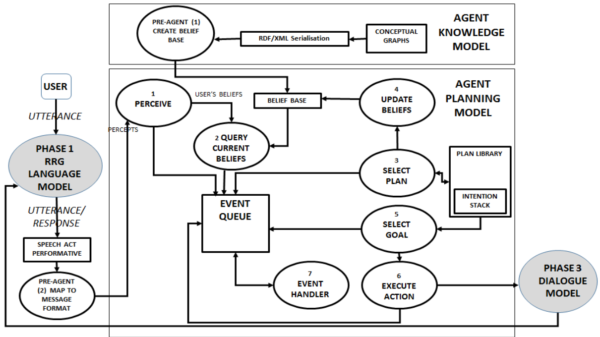
Figure 6: Design framework: Ling-CSA agent cognitive model.
