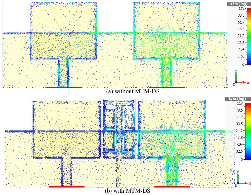
Fig. 12. Surface current density plots to validate the effect of MTM-DS at 10.65 GHz.
