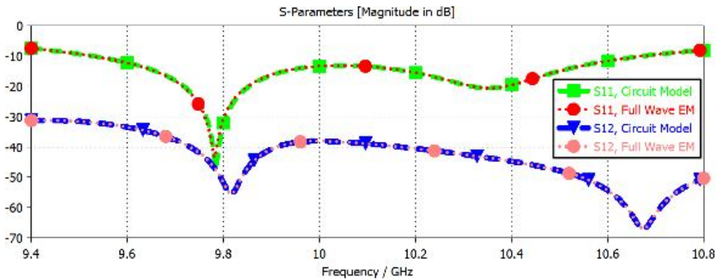
Fig. 10. Comparison of S-parameter response of the circuit and EM models for the 2×1 antenna array with MTM-DS.
