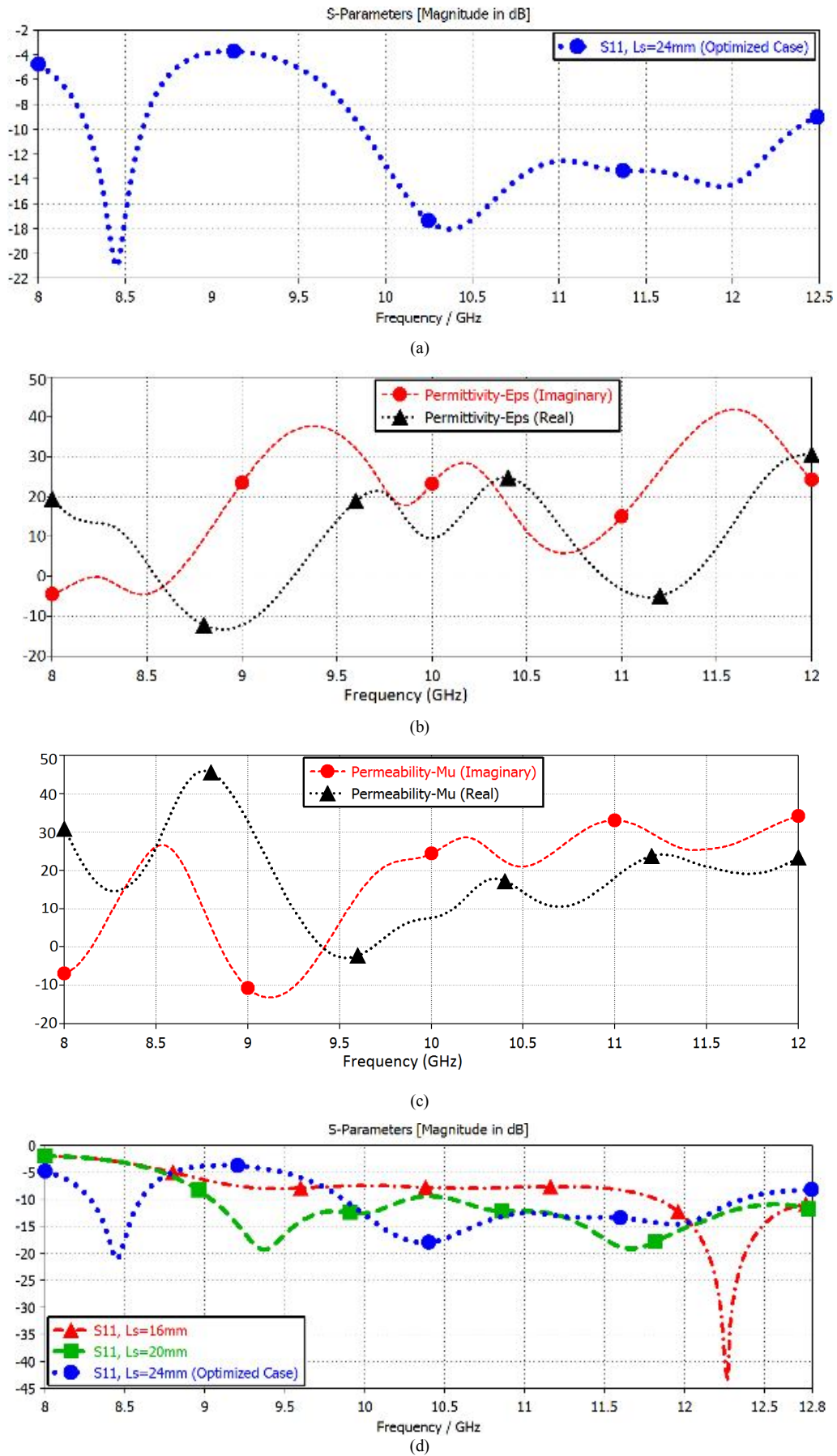
Fig. 7. MTM-DS response: (a) S_{11} , (b) permittivity (Eps), (c) permeability (Mu), and (d) S_{11} as a function of slit length ( L_s ).
