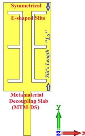
Fig. 6. The structure of the proposed metamaterial decoupling slab, where surface waves propagate along the x-axis, H||y , E||z .
