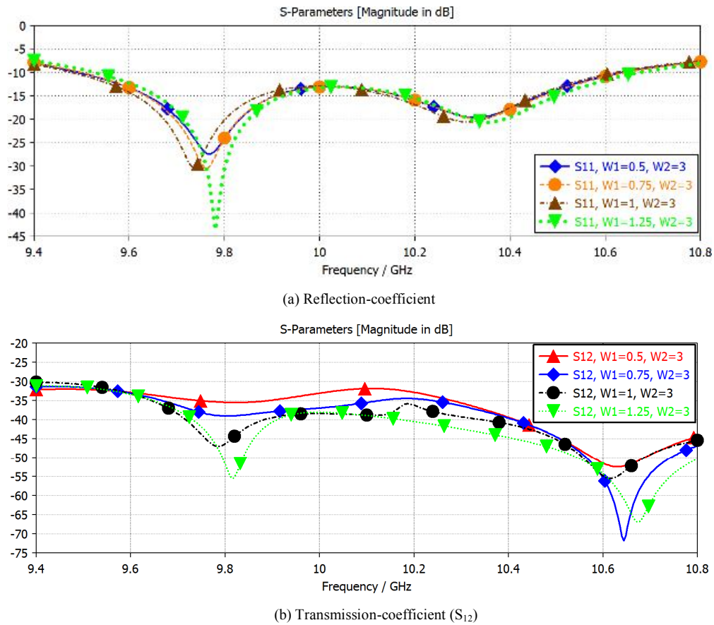
Fig. 13. Parametric study on slit width ( W_1 ) when the gap between the E-shaped slits is fixed at 3 mm.
