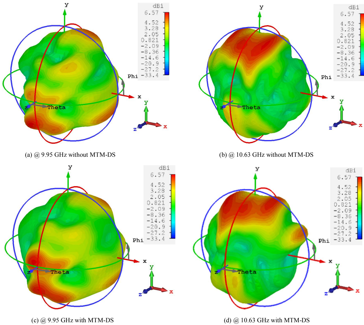
Fig. 18. 3D radiation patterns without and with MTM-DS at high impedance matching frequencies.
