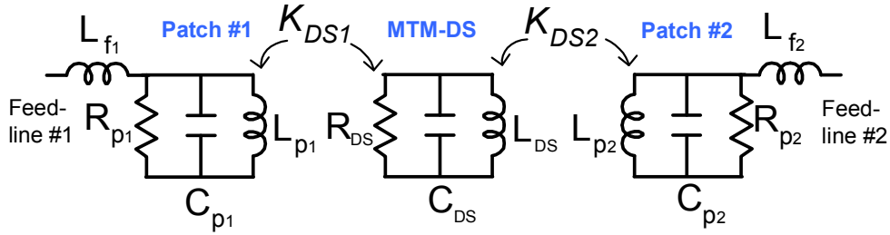
Fig. 9. Simplified equivalent circuit of two-element radiating patch with MTM-DS.
