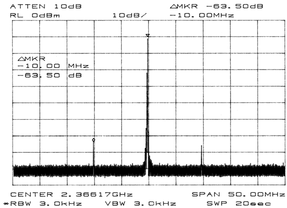
Figure 4.33 Measured spectrum of the AM modulation for a 10 MHz sinusoidal modulated signal.
