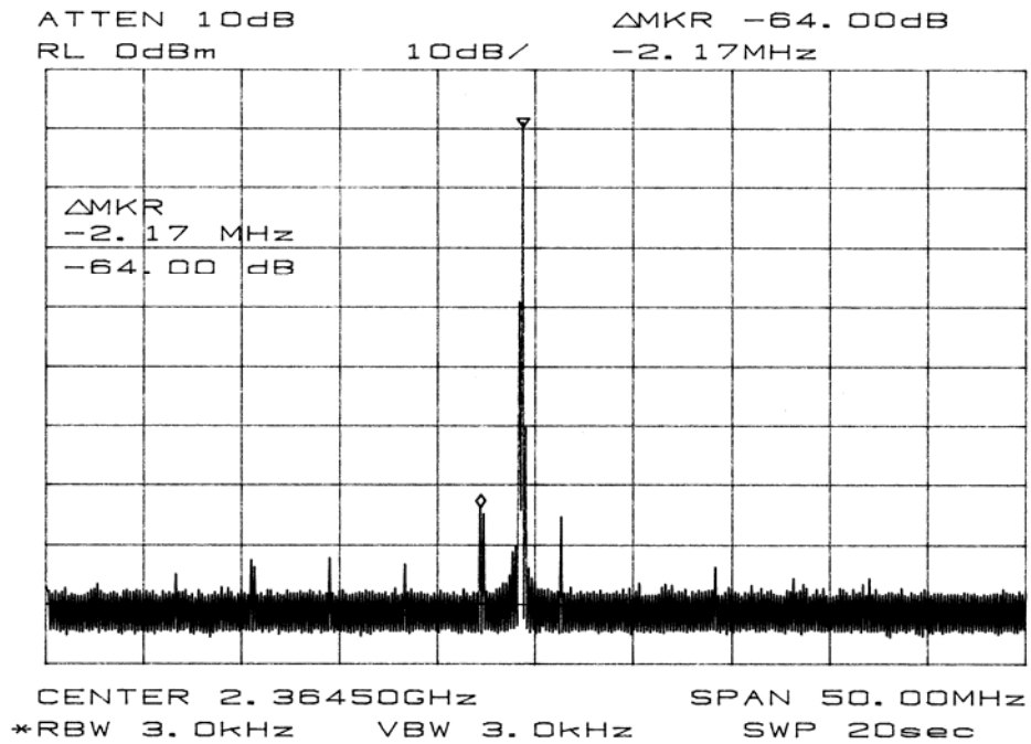
Figure 4.35 Measured spectrum of the ASK modulation for 2 MHz square wave.
