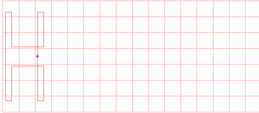
Figure 6.15 Folded loop antenna model using NEC Win Professional.
