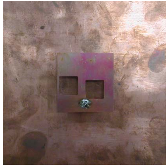
Figure 6.26 Photograph of a fabricated prototype antenna with two slots for CP.
