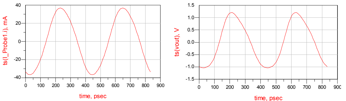
Figure 3.15 The drain output waveforms, current (left) and voltage (right).
