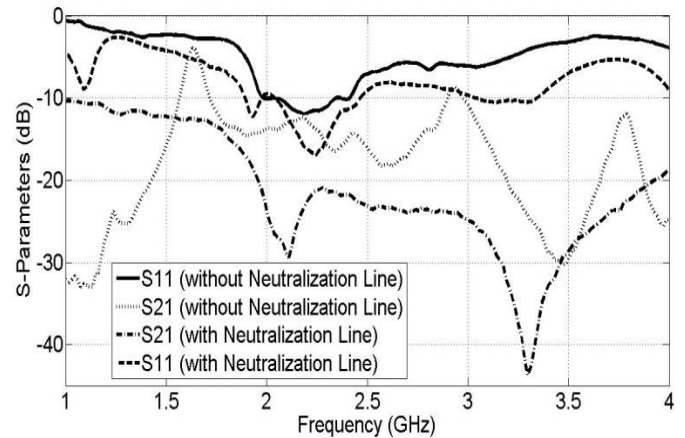
Figure 6. Measured S-parameters of the proposed antenna with and without the neutralization line.
