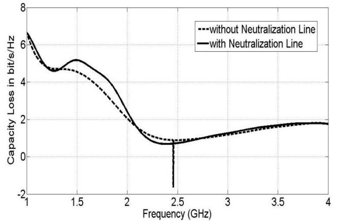
Figure 9. Simulated capacity loss of the proposed antenna with and without neutralization line.
