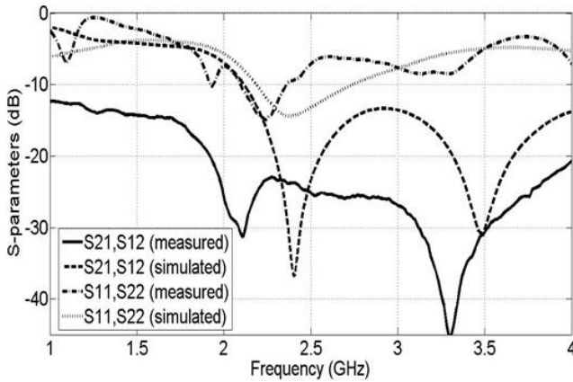
Figure 4. Comparative plot of s-parameters output for simulated and measured results for the proposed antenna with neutralization line.
