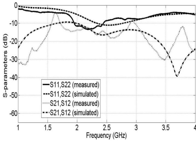
Figure 3. Comparative plot of s-parameters output for simulated and measured results for the proposed antenna without neutralization line.
