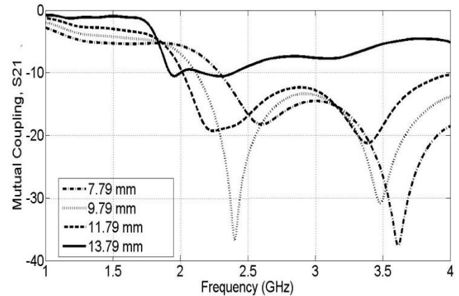
Figure 2. Simulated transmission coefficient, S_{21} of the various distance location of neutralization line.
