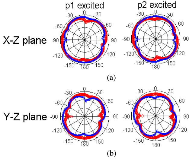
Figure 7. Simulated radiation patterns for the proposed antenna for two planes at 2.4 GHz; (a) X-Z plane. “xxxx” (blue) simulated cross-polarization, “oooo” (red) simulated co -polarization. (b) Y-Z plane. “xxxx” (blue) simulated co-polarization, “oooo” (red) simulated cross-polarization Port 1(left) excited and port 2(right) terminated in 50Ω.
