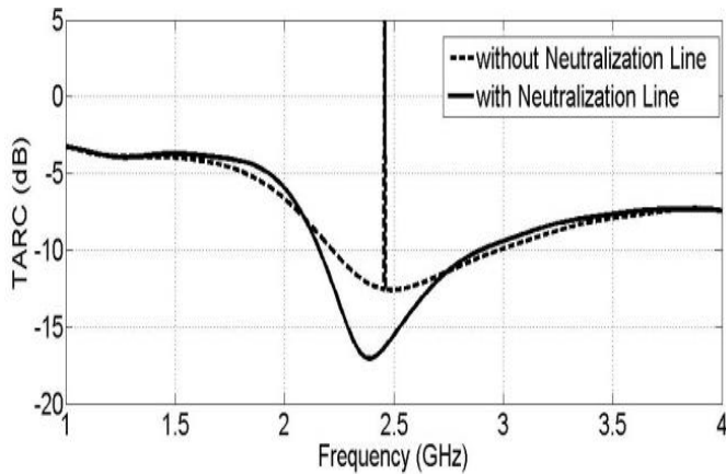
Figure 10. Simulated total active reflection coefficient of the proposed antenna with and without neutralization line.
