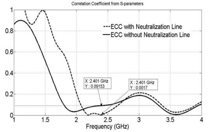
Figure 8. Simulated envelope correlation coefficient for the proposed antenna with and without neutralization line.
