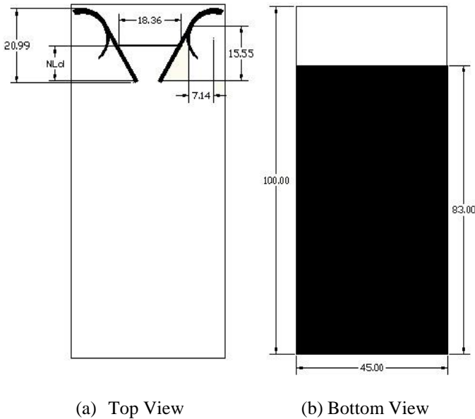
Figure 1. Geometry of the proposed antenna (in mm) (a) top view, and (b) Bottom view.
