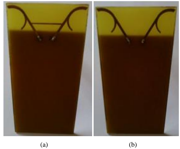
Figure 5. Practical prototype of the proposed antenna (a) with neutralization line (b) without the neutralization line.
