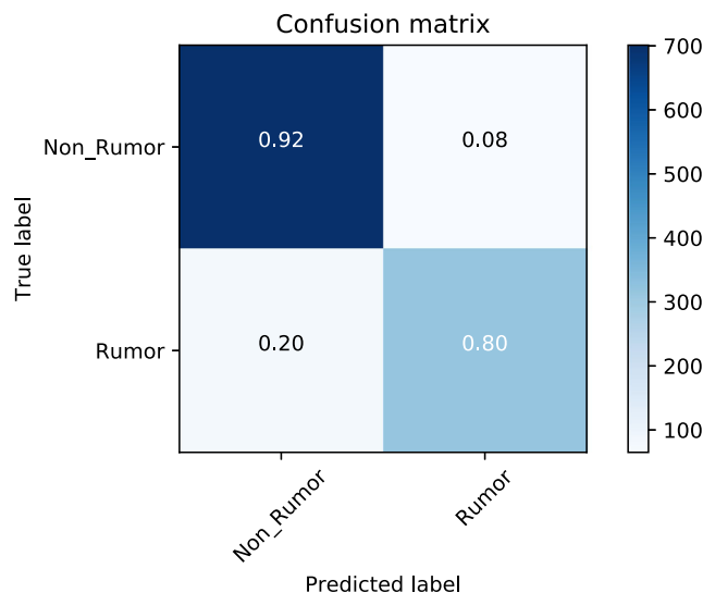
Fig. 6 Confusion matrix for fold-4 in case LSTM + Attention (Text + features)
