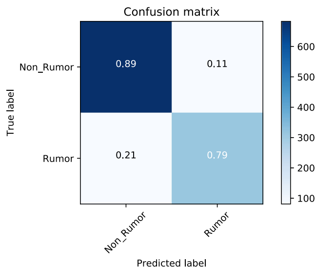
Fig. 7 Confusion matrix for fold-5 in case LSTM + Attention (Text + features)
