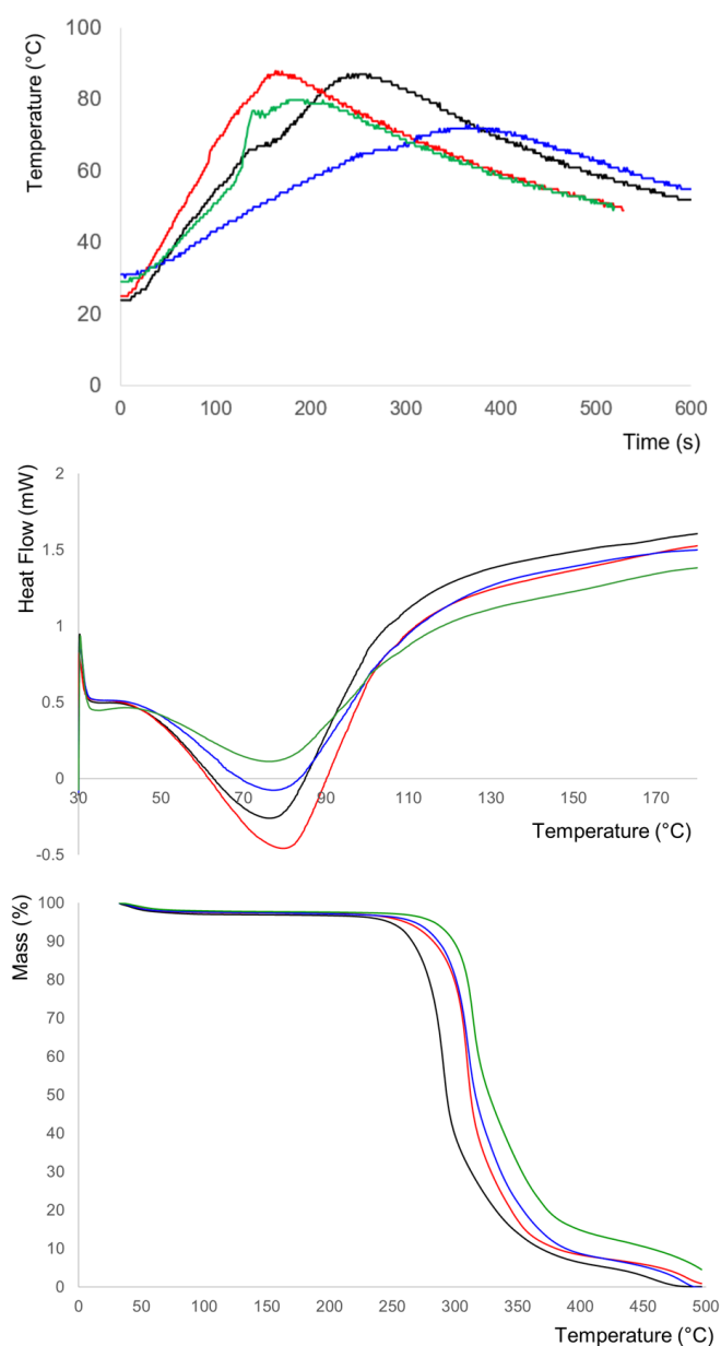
Figure 5: Heating profiles (top), representative DSC (centre) and TGA (bottom) traces for polymers synthesised with differing solvents and cross-linkers Black: Acetonitrile – EGDMA. Red: Chloroform – EGDMA. Blue: Acetonitrile – TRIM. Green: Chloroform – TRIM.
