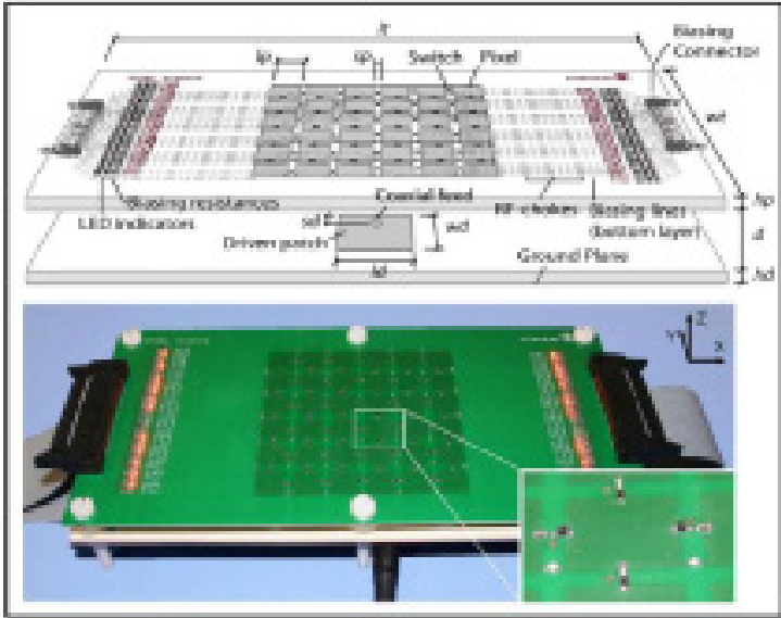
Figure 9: Schematic of the multi-functional reconfigurable antenna [99].
