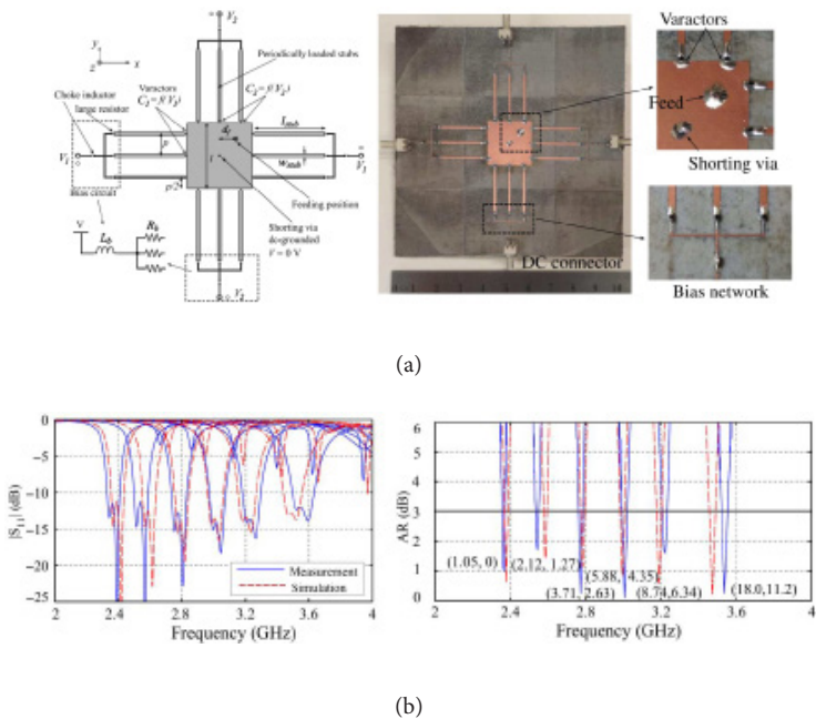
Figure 7: (a) Configuration and (b) performance of the frequency and polarization reconfigurable antenna in [87].
