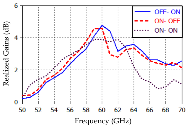
Figure 12: Realized gain in different states of switches for the proposed antenna
