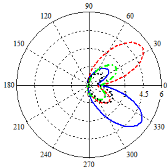
Figure 3: Radiation pattern at yz-plane for different angles of \phi using the metal tab as switch ( \phi=0 : dotted line, \phi =30 : solid line, \phi=150 : dashed line and \phi=180 : dotted/dashed line).
