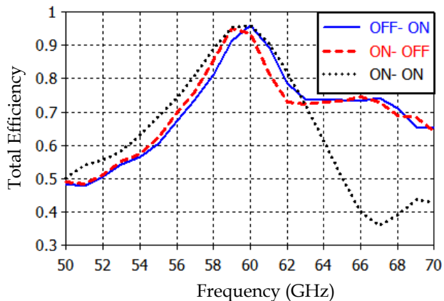
Figure 13: Total efficiency in different states of switches for the proposed antenna
