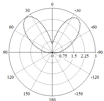
Figure 8: Radiation pattern at yz-plane in the on-on state
