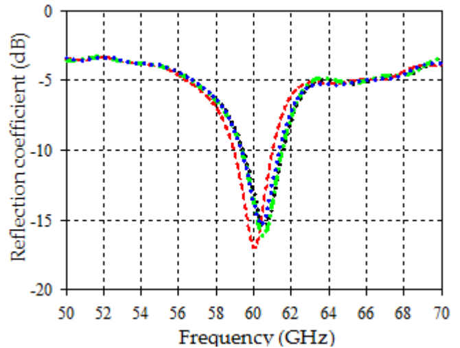
Figure 2: The frequency response of the input reflection coefficient for different angles of \phi using the metal tab as switch ( \phi=0 : dotted line, \phi =30 : solid line, \phi=150 : dashed line and \phi=180 : dotted/dashed line).
