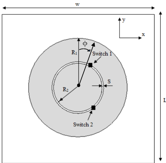
Figure 1: The geometry structure of the proposed antenna.
