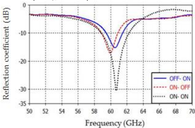
Figure 5: Simulation results for the proposed antenna for different states of switching.
