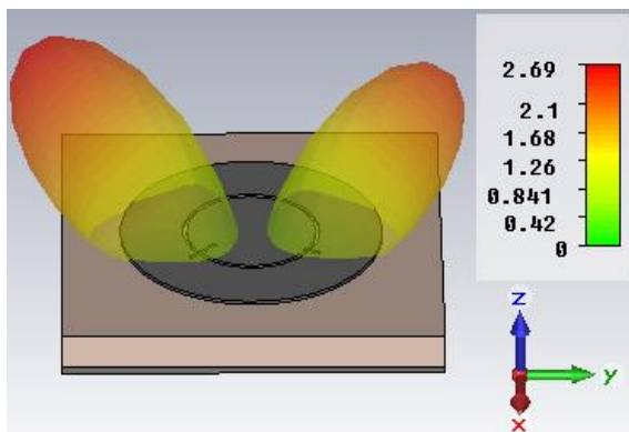
Figure 11: 3D radiation pattern in the on-on state.
