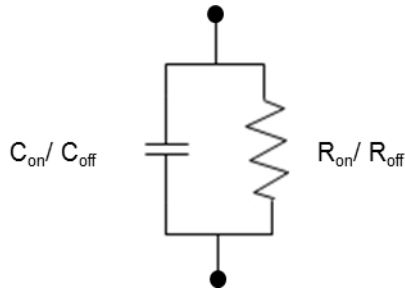
Figure 4: Simplified electrical model of the NMOS transistor switch in ON and OFF states.
