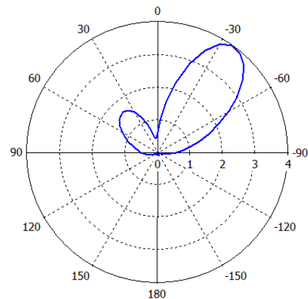
Figure 7: The radiation pattern at yz-plane in the off-on state.
