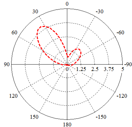
Figure 6: Radiation pattern at yz-plane in the on-off state
