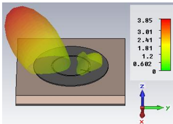
Fig. 10. 3D radiation pattern in the off-on state
