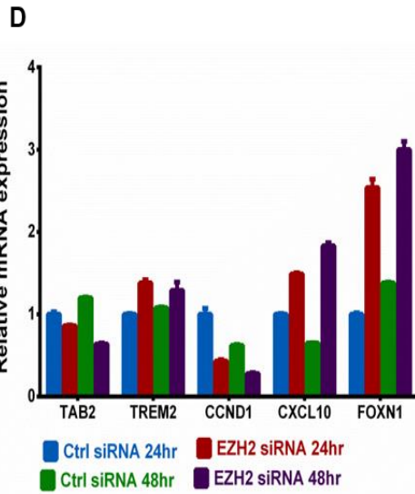
Figure 3.2.5. EZH2 depletion mediates complex changes in gene expression program in primary keratinocytes. (A) Gene Ontology (GO) terms enriched in EZH2-depleted NHEKs (DAVID 6.8
