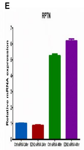
Figure 3.2.5. EZH2 depletion mediates complex changes in gene expression program in primary keratinocytes. (A) Gene Ontology (GO) terms enriched in EZH2-depleted NHEKs (DAVID 6.8
