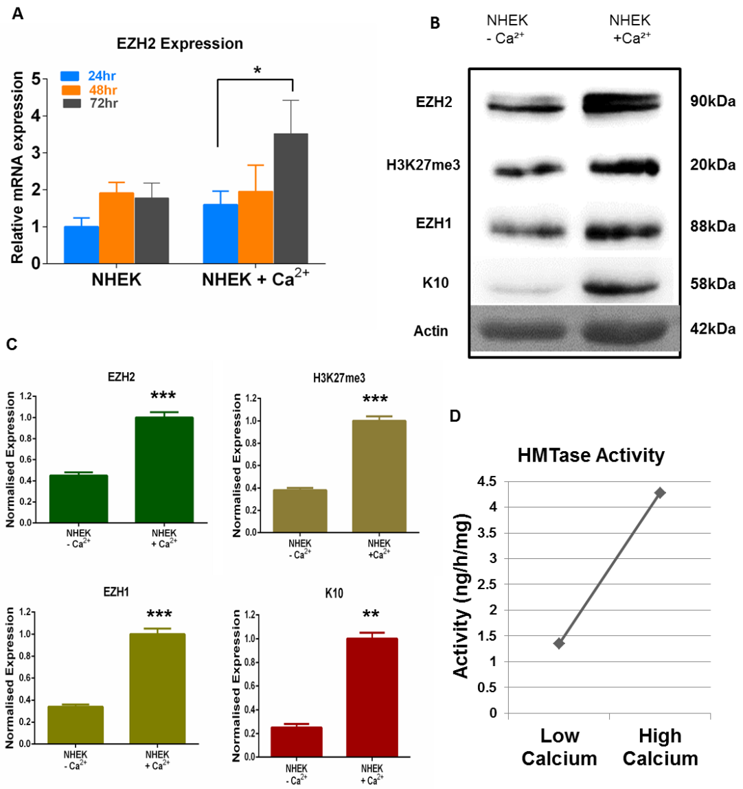
Figure 3.2.2. EZH2 expression and enzymatic activity increases in differentiating keratinocytes in vitro . (A) RT-qPCR showing upregulation of EZH2 in differentiating keratinocytes during Ca 2+ -induced differentiation (Mean±SD; n=3; *P<0.05). (B-C) Western blot and densitometric analysis showing increased EZH2, H3K27me3, EZH1 and K10 protein levels in differentiating keratinocytes during Ca 2+ -induced differentiation. Actin was used as a loading control (Mean±SD; n=3, **P<0.01, ***P<0.001). (D) HMTase activity assay showing increased HMTase activity in differentiating keratinocytes during Ca 2+ -induced differentiation. NHEK - Normal human epidermal keratinocytes. HMTase – Histone Methyltransferase
