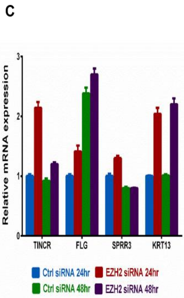
Figure 3.2.5. EZH2 depletion mediates complex changes in gene expression program in primary keratinocytes. (A) Gene Ontology (GO) terms enriched in EZH2-depleted NHEKs (DAVID 6.8
