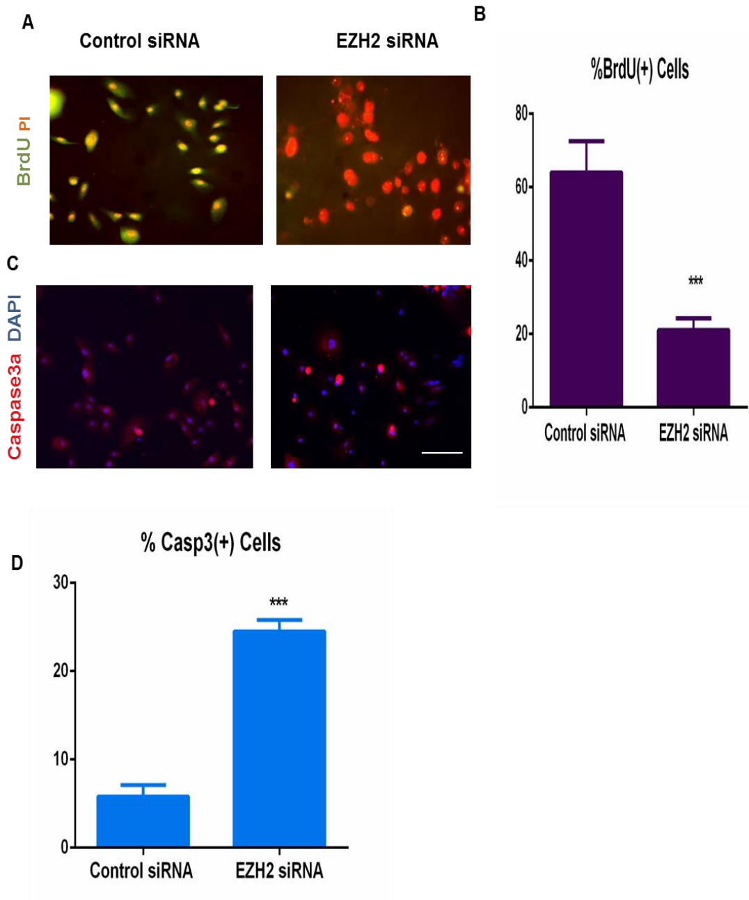
Figure 3.2.9. Loss of EZH2 leads to reduced proliferation and induced apoptosis in NHEKs (A) BrdU staining showing reduced proliferation in EZH2 deficient NHEKs (B) Quantification of percentage of BrdU(+) NHEKs (Mean±SD; n=5, ***P<0.001) (C) Activated Caspase 3 (Caspase3a) staining showing increased apoptosis in EZH2 deficient NHEKs (D) Quantification of percentage of Casp3(+) NHEKs (Mean±SD; n=5, ***P<0.001). Scale bar: 100µm. PI - Propidium iodide
