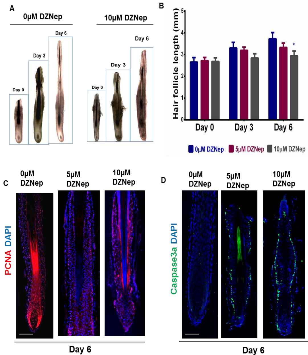
Figure 4.2.2. Inhibition of EZH2 activity in human hair follicles ex vivo results in hair growth retardation. (A-B) Inhibition of EZH2 activity with a selective small molecule, DZNep, causes a dose-dependent retardation of hair growth ex vivo . (Mean±SD, n= 3 donors and 6 HF for each treatment group, P* < 0.05) (C) Immunohistochemical staining with anti-PCNA antibody showing a dose-dependent decrease in proliferation (D) Immunohistochemical staining with anti-Caspase 3a antibody showing a dose-dependent increase in apoptosis in the ORS. Scale bars: 50µM
