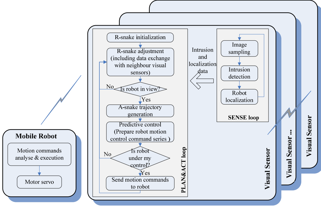
Fig. 8. Experiment system components and functional modules
