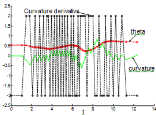
(c) Planned curvature derivative, curvature and orientation
