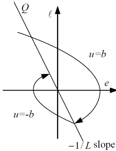
Fig. 5. Phase track of e and \ell
