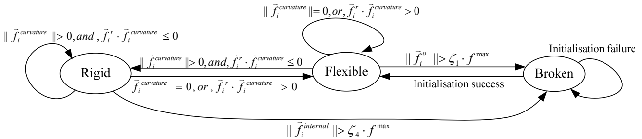
Fig.2. State machine for state transition
