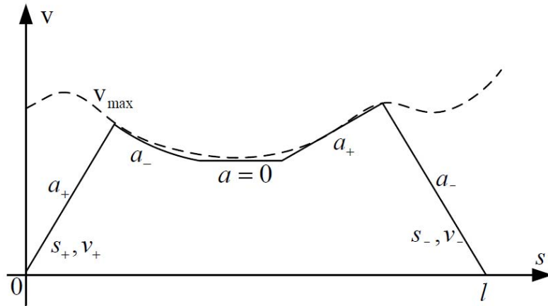
Fig.7. Rolling window optimization for trajectory generation (assume v_{r,0} = 0 )
