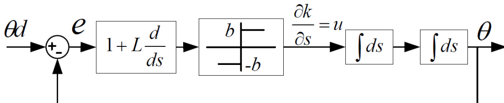
Fig. 4. Heading direction generation of an A-snake
