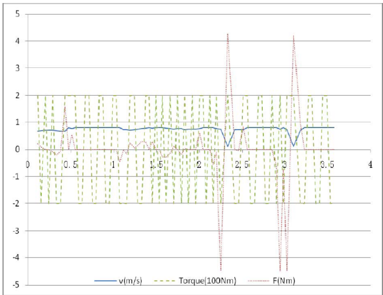
Fig. 12. Robot control and velocity (driving force F_d : dot; steering torque \tau : dashed; velocity v : solid)
