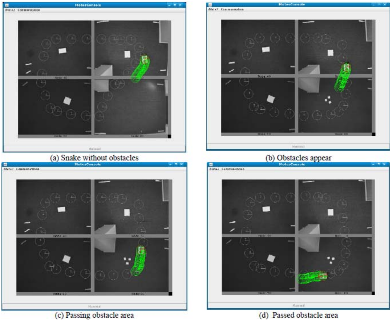
Fig.11. The real time experiments of robot control by a visual sensor network
