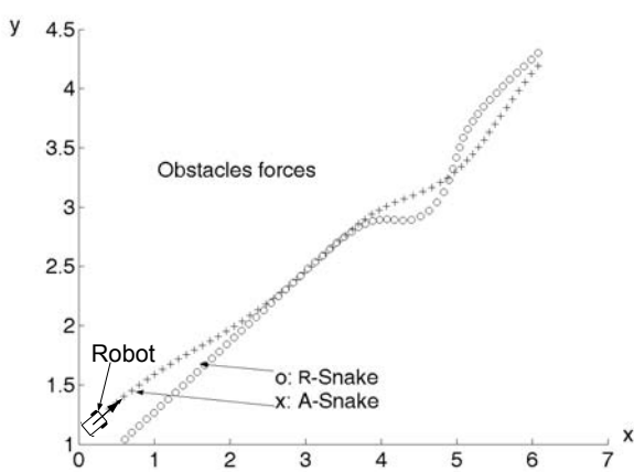
(a) Deformable snake with A-snake
