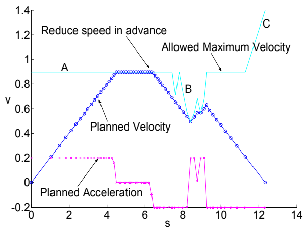
(b) Maximum velocity, planned velocity and acceleration
