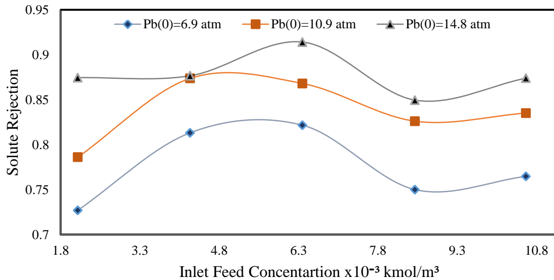
Figure 5. Solute rejection versus inlet feed concentration for three different inlet feed pressure, inlet feed conditions 3.333 \times 10^{-4} m 3 /s and (32.2 – 34.5 °C)
