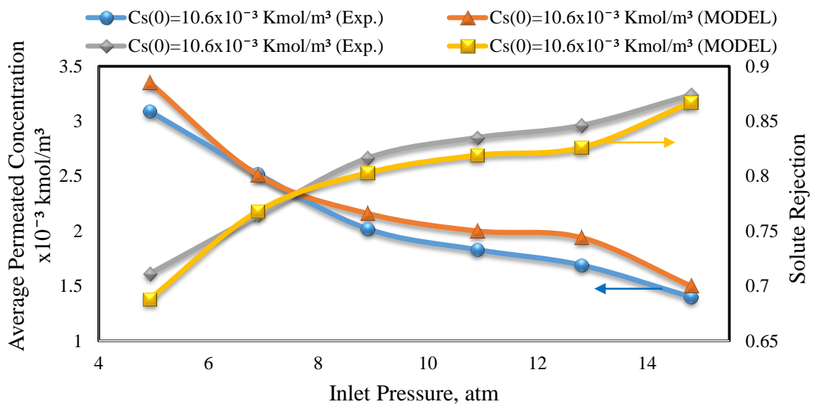
Figure 1. Comparison of theoretical and experimental results of solute rejection and average permeate concentration
