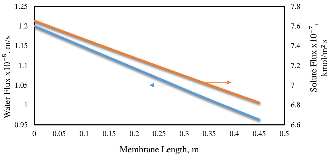
Figure 4. Water and solute fluxes variation along the membrane length, inlet feed conditions ( 3.333 \times 10^{-4} \text{ m}^3/\text{s} , 8.5 \times 10^{-3} \text{ kmol}/\text{m}^3 , 10.9 atm and 32.2 °C)
