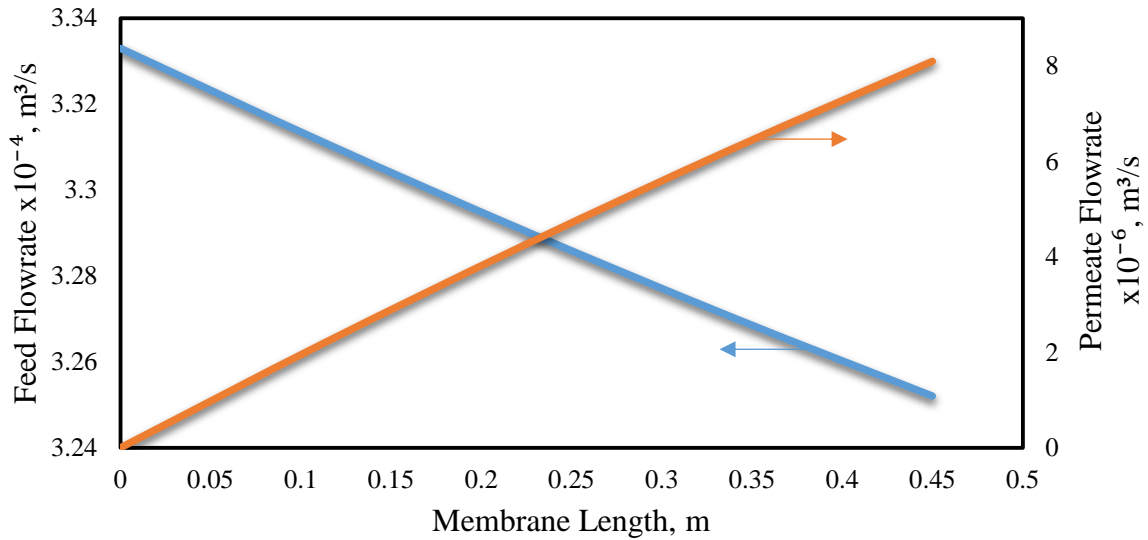
Figure 3. Feed and permeate flow rates variation along the membrane length, inlet feed conditions ( 3.333 \times 10^{-4} \text{ m}^3/\text{s} , 8.5 \times 10^{-3} \text{ kmol}/\text{m}^3 , 10.9 atm and 32.2 °C)
