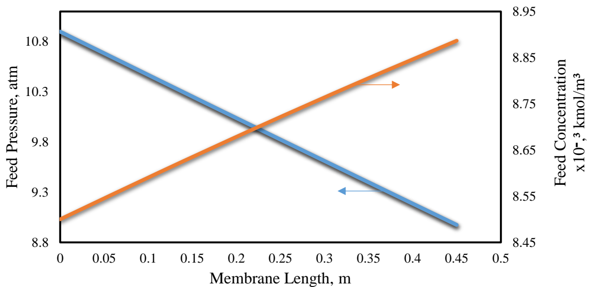
Figure 2. Feed pressure and concentration variation along the membrane length, inlet feed conditions ( 3.333 \times 10^{-4} m 3 /s, 8.5 \times 10^{-3} kmol/m 3 , 10.9 atm and 32.2 °C)
