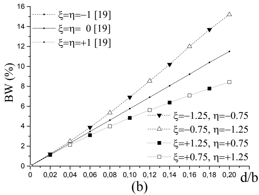
Fig. 3: Chirality effect on the (a) real part of resonant frequency, (b) half-power bandwidth; for (\bar{\xi} \neq \bar{\eta}, \bar{\xi} \neq 0 and \bar{\eta} \neq 0) , a=1.5\text{cm} , b=1\text{cm} , \epsilon_r=2.35 .
