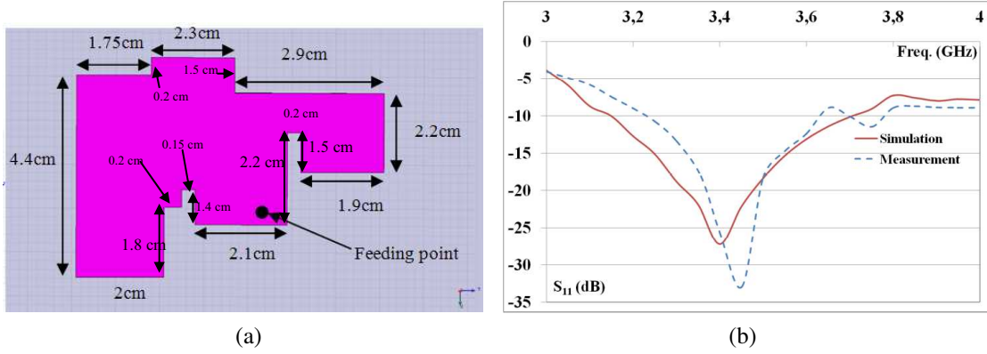
Figure 3. Modified E-shaped patch antenna; (a) Dimension description. (b) S_{11} parameter.
