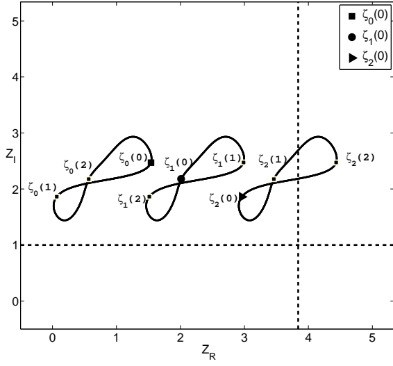
Figure 6: Paths of the zeros of the analytic representation of the state |\lambda^r\rangle|g\rangle . The period is T = 3 . The state |g\rangle is defined through the zeros at t = 0 given in Eq.(37). Dotted lines show a cell, which is a square with each side equal to 4.34
