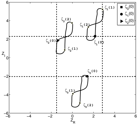
Figure 7: Paths of the zeros of the analytic representation of the state [\mathcal{D}(1,1)]^l|g\rangle . The period is T = 3 . The state |g\rangle is defined through the zeros at t = 0 given in Eq.(39). Dotted lines show a cell, which is a square with each side equal to 4.34
