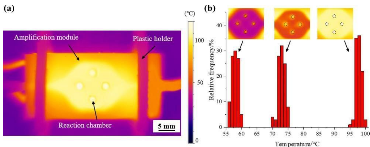
Fig. 4 Temperature measurement with a thermal imaging camera. (a): a thermograph of the amplification module taken with a thermal imaging camera. (b): the frequency distribution histogram of the temperature in the reaction chambers at setting temperatures of 58 °C, 72 °C, and 98 °C
