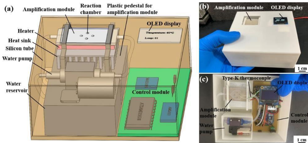
Fig. 1 Overview of the proposed PCR microdevice. (a): a schematic drawing illustrating the design of the PCR microdevice. (b): photo- graph of the wholly assembled PCR microdevice. (c) interior photo- graph of the assembled PCR microdevice.
