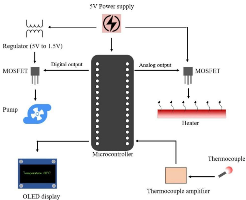
Fig. 2 Schematic diagram of the control module
