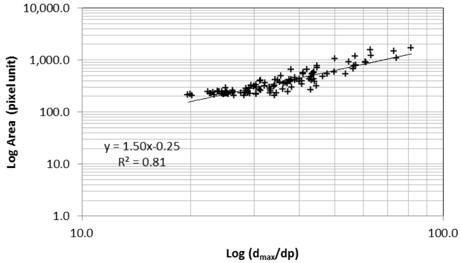
4 Figure S.I.1 –log-log plot of area versus relative longest length based on pixel size.
