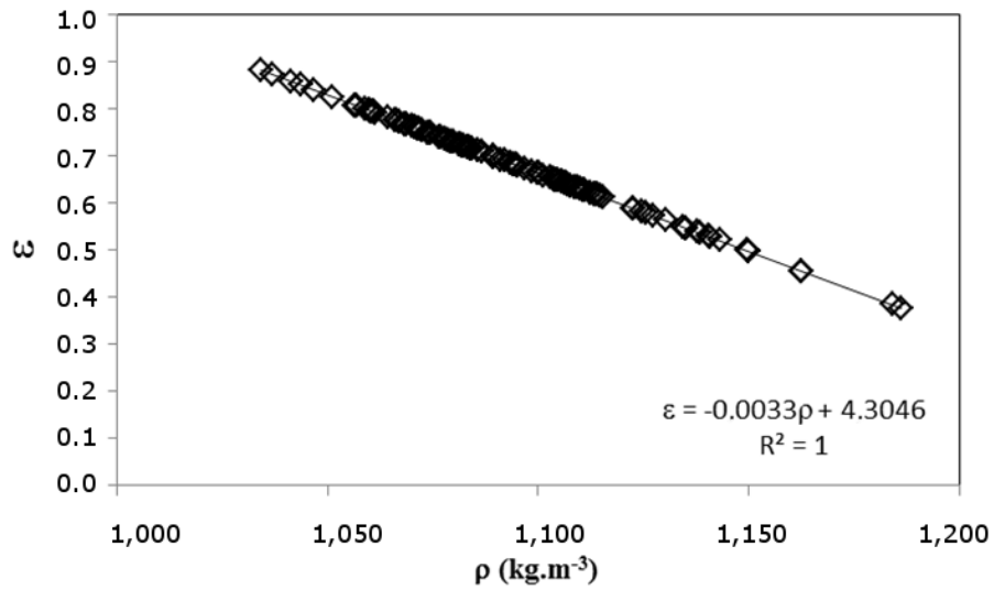
7 Figure S.I.2 – Aggregate porosity ( \epsilon ) as a function of density.
