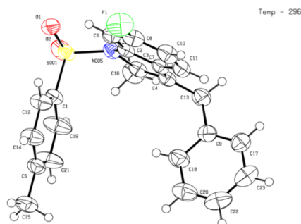
Figure 1. X-ray crystal structure of 8o
