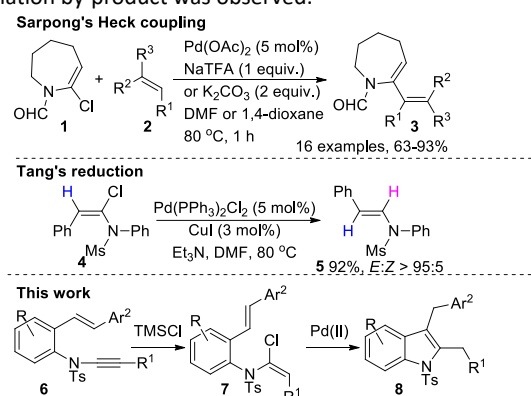
Scheme 1. Heck coupling and reduction of Chloro-enamides.
