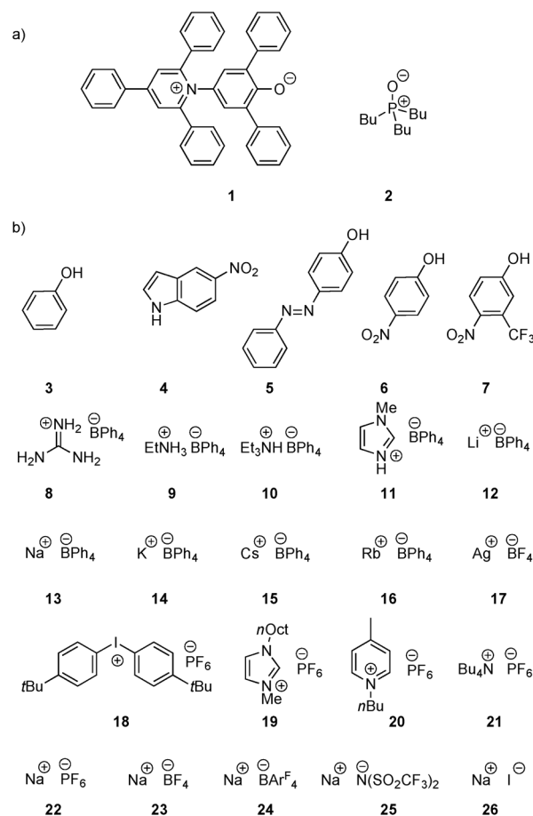
Scheme 1 (a) H-Bond acceptors and (b) cations ( \text{Ar}^{\text{F}} = 3,5\text{-bis(trifluoromethyl)phenyl} , \text{R} = 2\text{-ethylhexyl} , 12 is the tris(1,2-dimethoxyethane) adduct).
