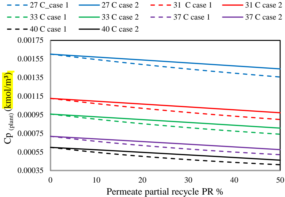
Fig. 6. The impact of plant feed temperature on the total plant product concentration of permeate recycle scheme of cases 1 and 2 (plant operating conditions of case 1: 6.226E-3 kmol/m 3 , 5.166E-4 m 3 /s, 15 atm and variable plant feed temperature and plant operating parameters of case 2: 6.226E-3 kmol/m 3 , 15 atm and variable plant feed flow rate and temperature)
