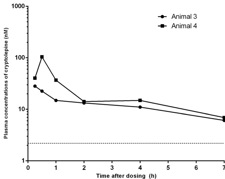
Fig. 5 Plasma concentration-time profiles of cryptolepine after single oral (5 mg/kg) administration to Sprague Dawley rats. The lower dotted line indicates the LLOQ (2.2 nM) of LC-MS/MS method for quantifying cryptolepine in rat plasma
