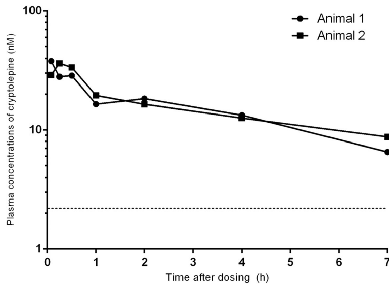
Fig. 4 Plasma concentration-time profiles of cryptolepine after single intravenous (1 mg/kg) administrations to Sprague Dawley rats. The lower dotted line indicates the LLOQ (2.2 nM) of LC-MS/MS method for quantifying cryptolepine in rat plasma
