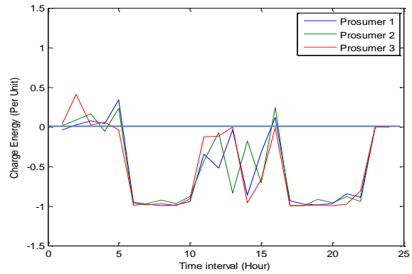
Fig. 11. Battery charge.
