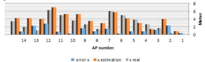
Figure 4: Comparison between the real and estimated values of x
