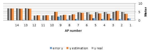
Figure 5: Comparison between the real and estimated values of y.
